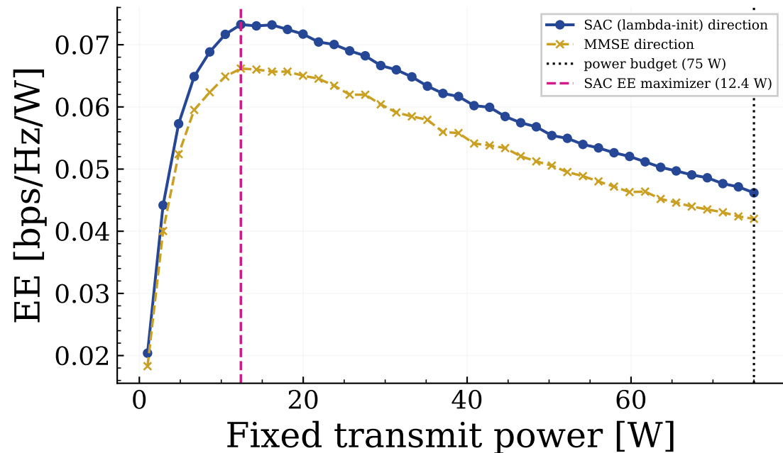
SAC (lambda-init) vs. MMSE direction, CSIT error bound=0.05
