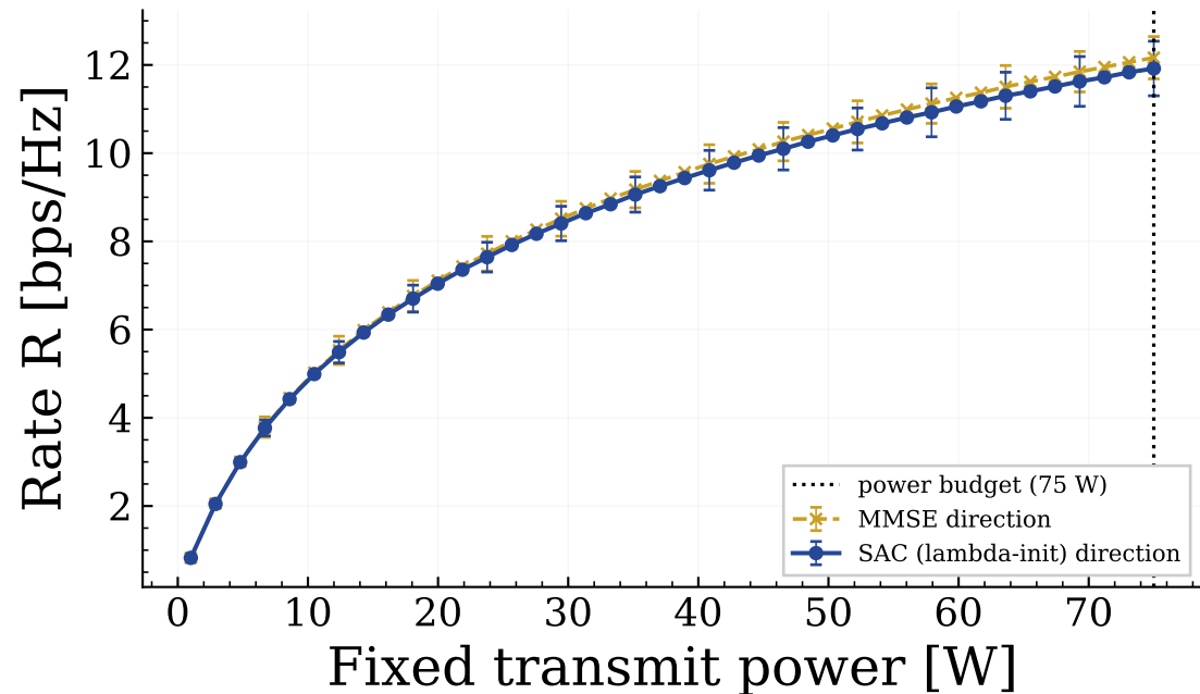
Rate vs. transmit power, perfect CSIT
