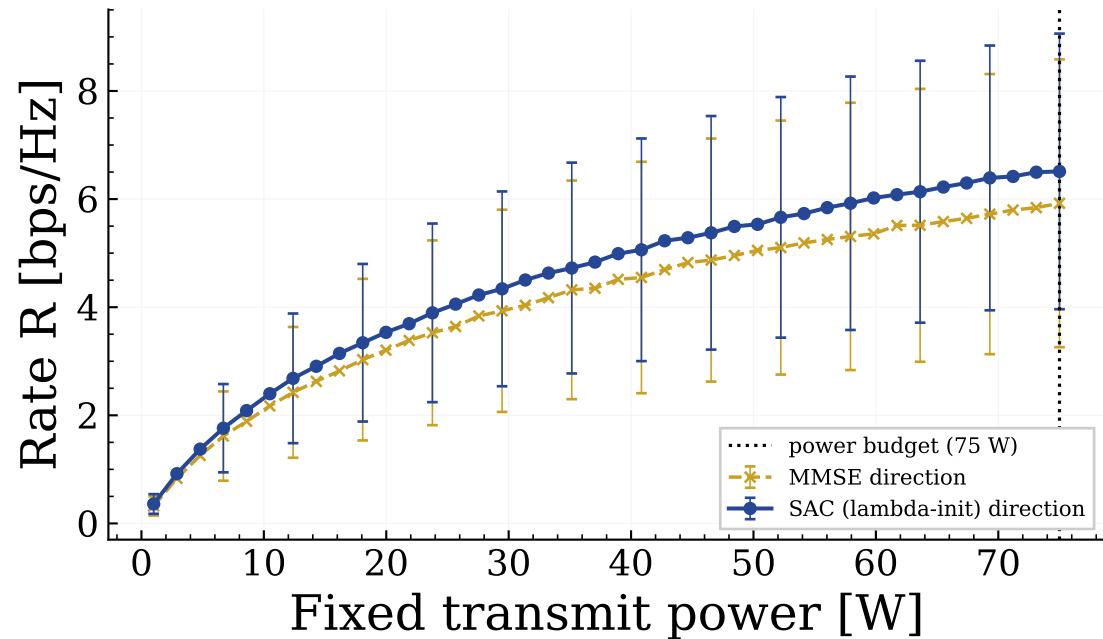
Rate vs. transmit power, CSIT error bound=0.05
