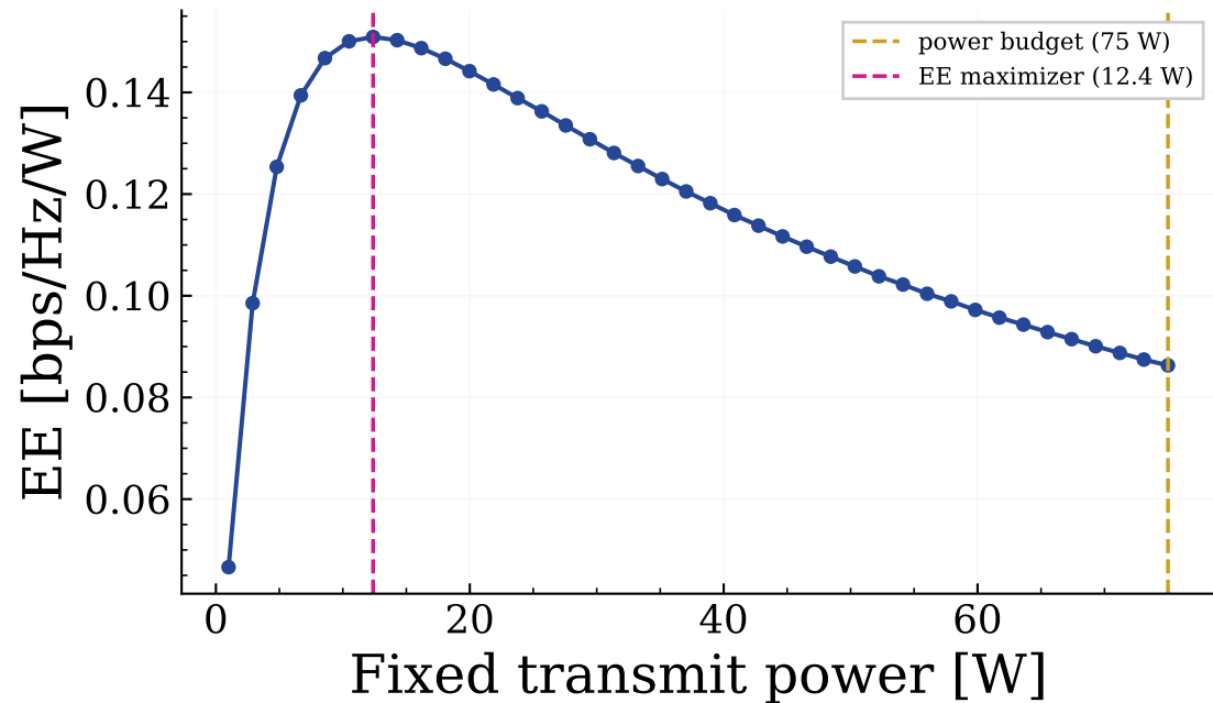
MMSE direction, CSIT error bound=0
