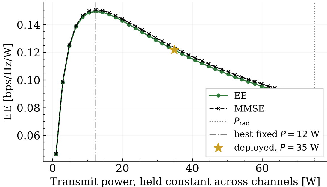
EE vs. constant transmit power, \Delta\varepsilon = 0
