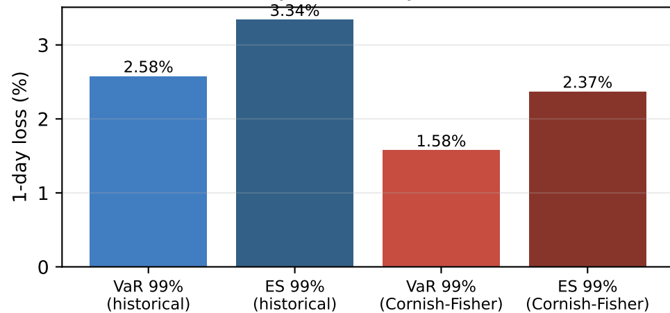
99% 1-day VaR / Expected Shortfall, carry sleeve daily returns
