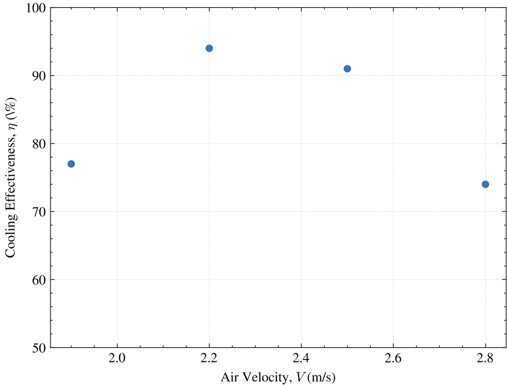
Effectiveness vs Fan Velocity
