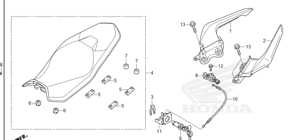
F-23 SEAT
