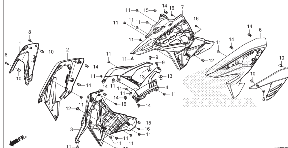
F-22 MIDDLE COWL
