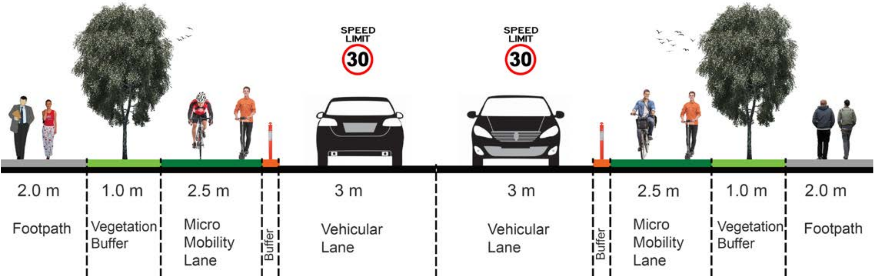
Section (NTS) Road Section (image source: Anagha Khude)
