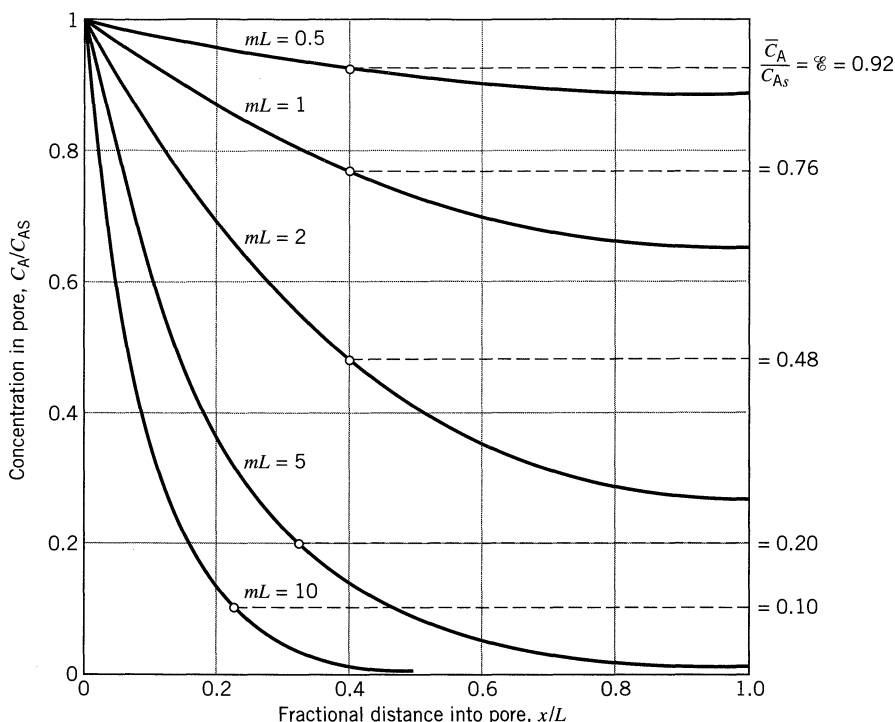
Figure 18.4 Distribution and average value of reactant concentration within a catalyst pore as a function of the parameter mL = L\sqrt{k/D}
