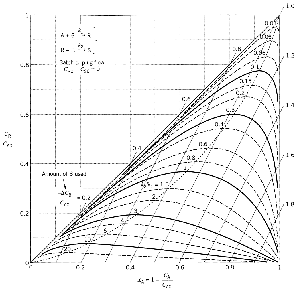
Figure 8.13 Distribution of materials in a batch or plug flow reactor for the elementary series-parallel reactions
