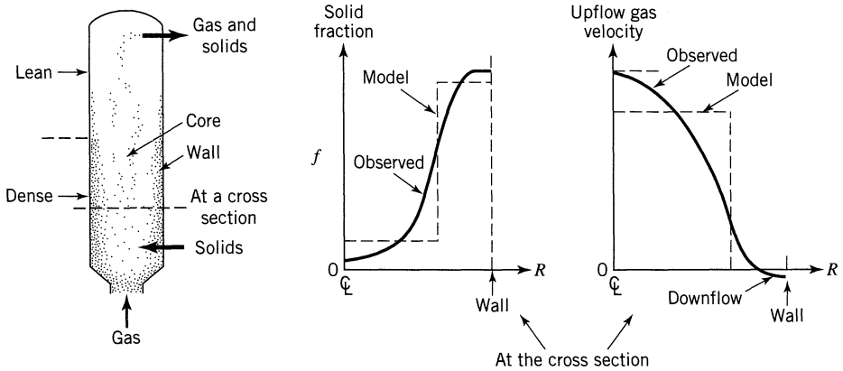
Figure 20.15 Behavior of a FF bed.
