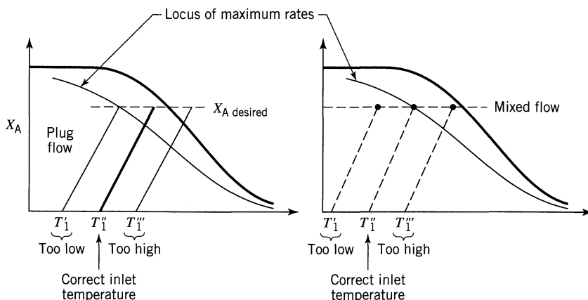
Figure 9.9 Best location for the adiabatic operating line. For plug flow, a trial and error search is needed to find this line; for mixed flow, no search is needed.
