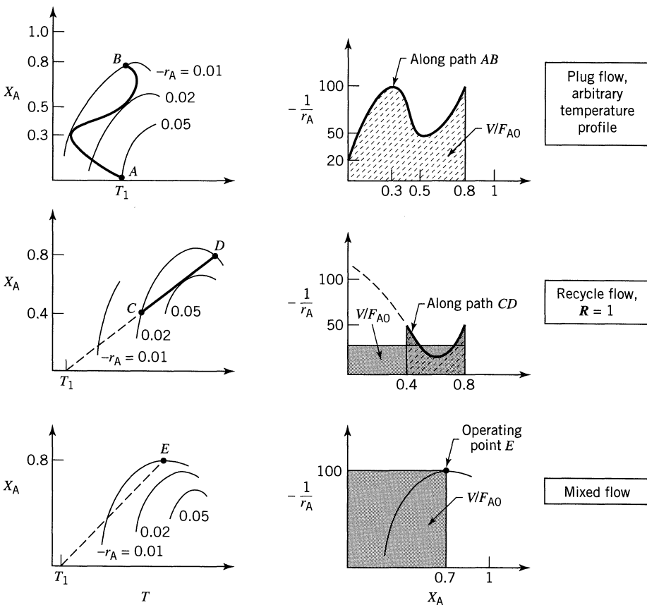
Figure 9.4 Finding the reactor size for different types of flow and for a feed temperature T_1 .
