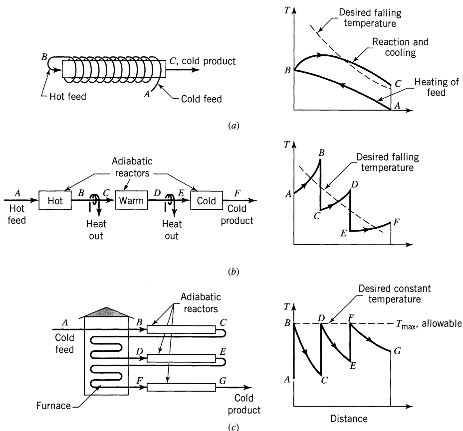
Figure 9.12 Ways of approaching the ideal temperature profile with heat exchange: (a) and (b) exothermic reaction; (c) endothermic reaction.
