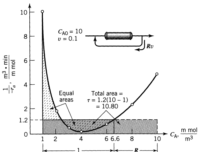
Figure E6.3a Plug flow with recycle.
