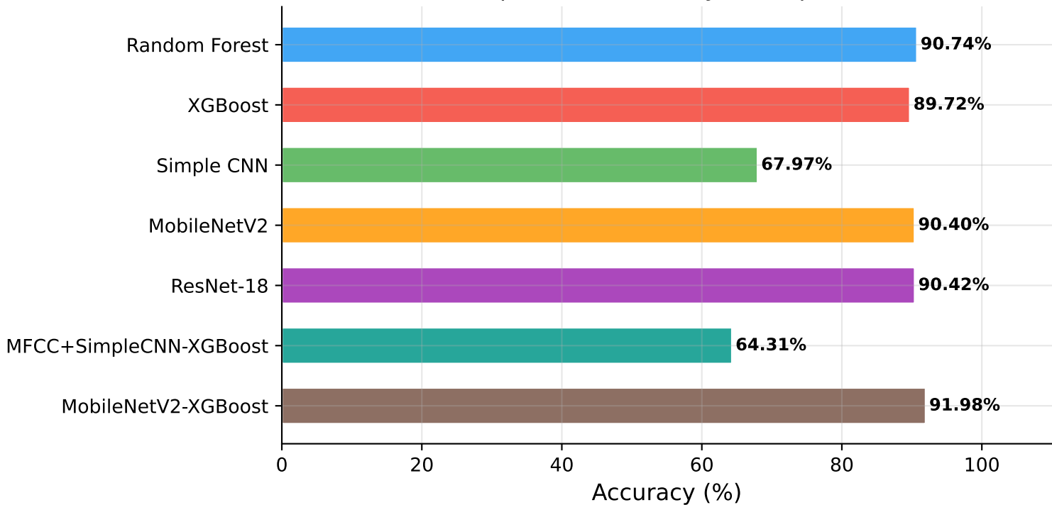
Model Comparison: Accuracy (ASVspoof 2019 LA)
