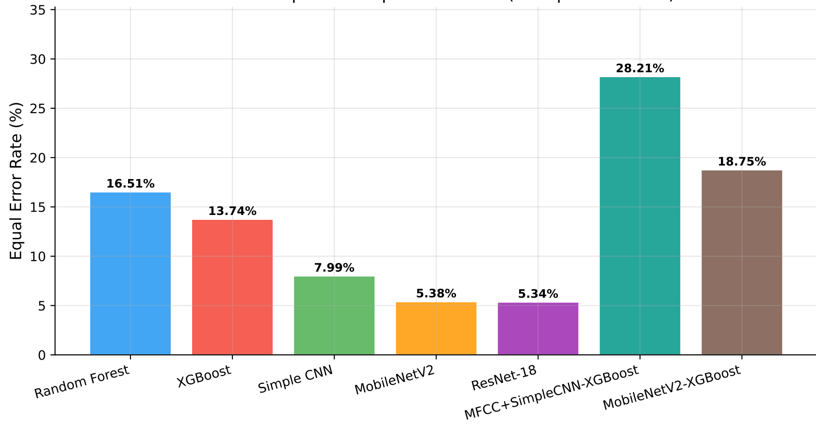
Model Comparison: Equal Error Rate (ASVspoof 2019 LA)
