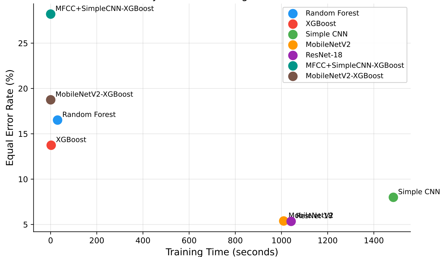
Efficiency Frontier: Training Runtime vs. EER
