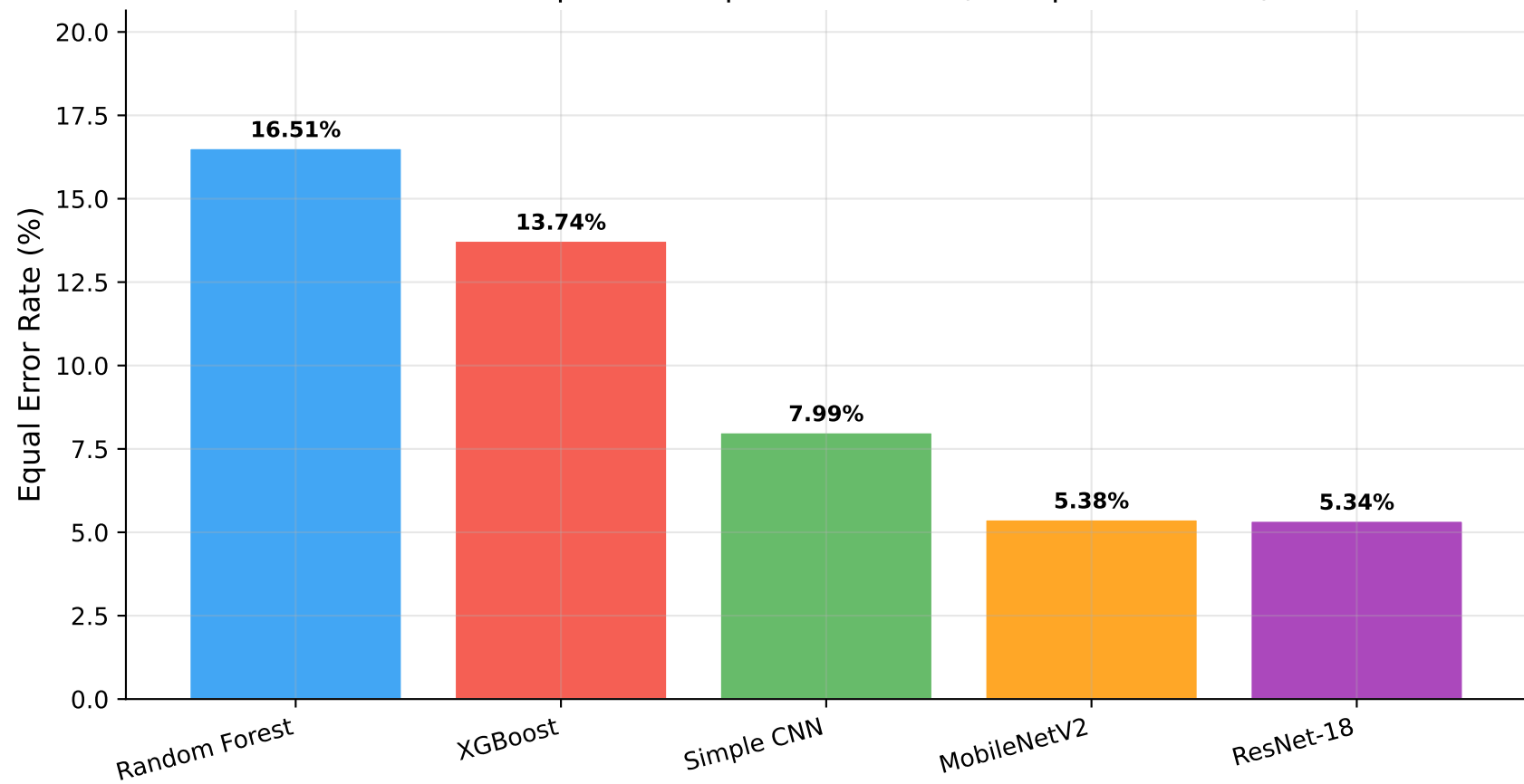
Model Comparison: Equal Error Rate (ASVspoof 2019 LA)
