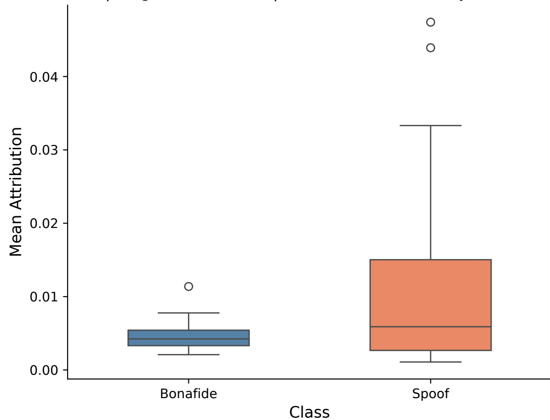
|Integrated Gradients| — Mean Attribution by Class
