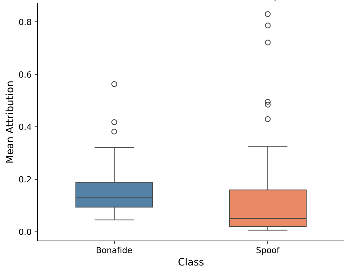
Occlusion (50ms) — Mean Attribution by Class
