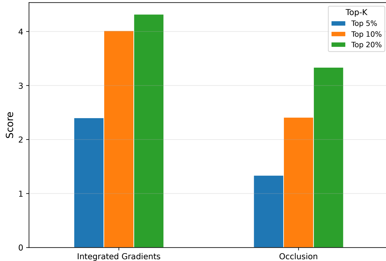
Comprehensiveness ( \uparrow = more faithful)
