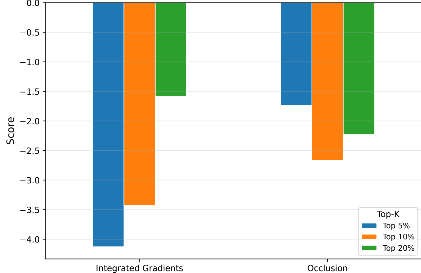
Sufficiency ( \uparrow = more faithful)
