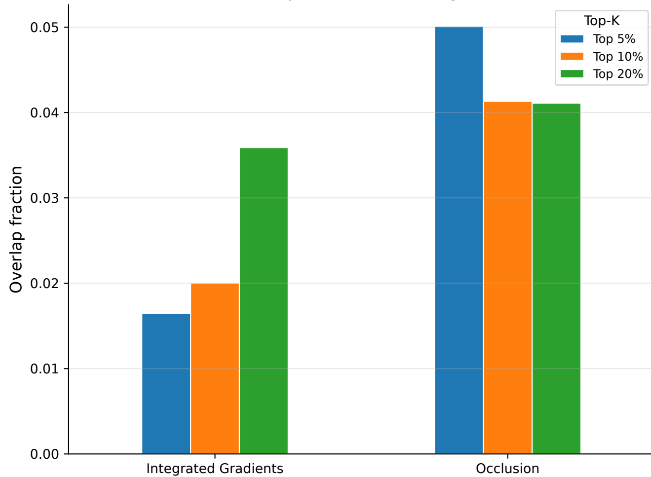
Fraction of Top-K Attribution Falling in Silence
