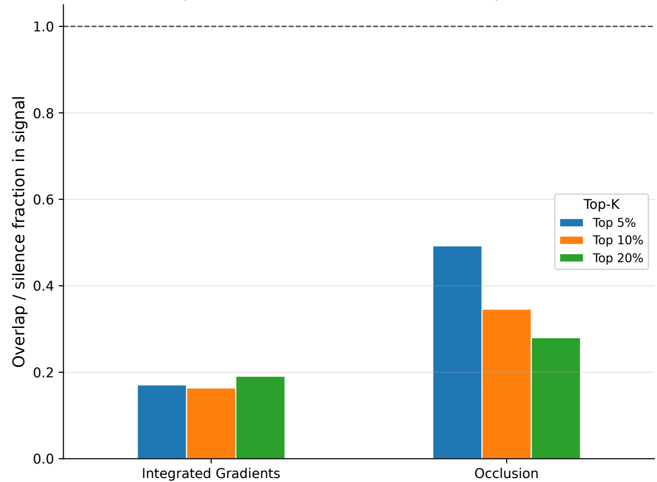
Overlap Relative to Chance (1.0 = no silence preference)
