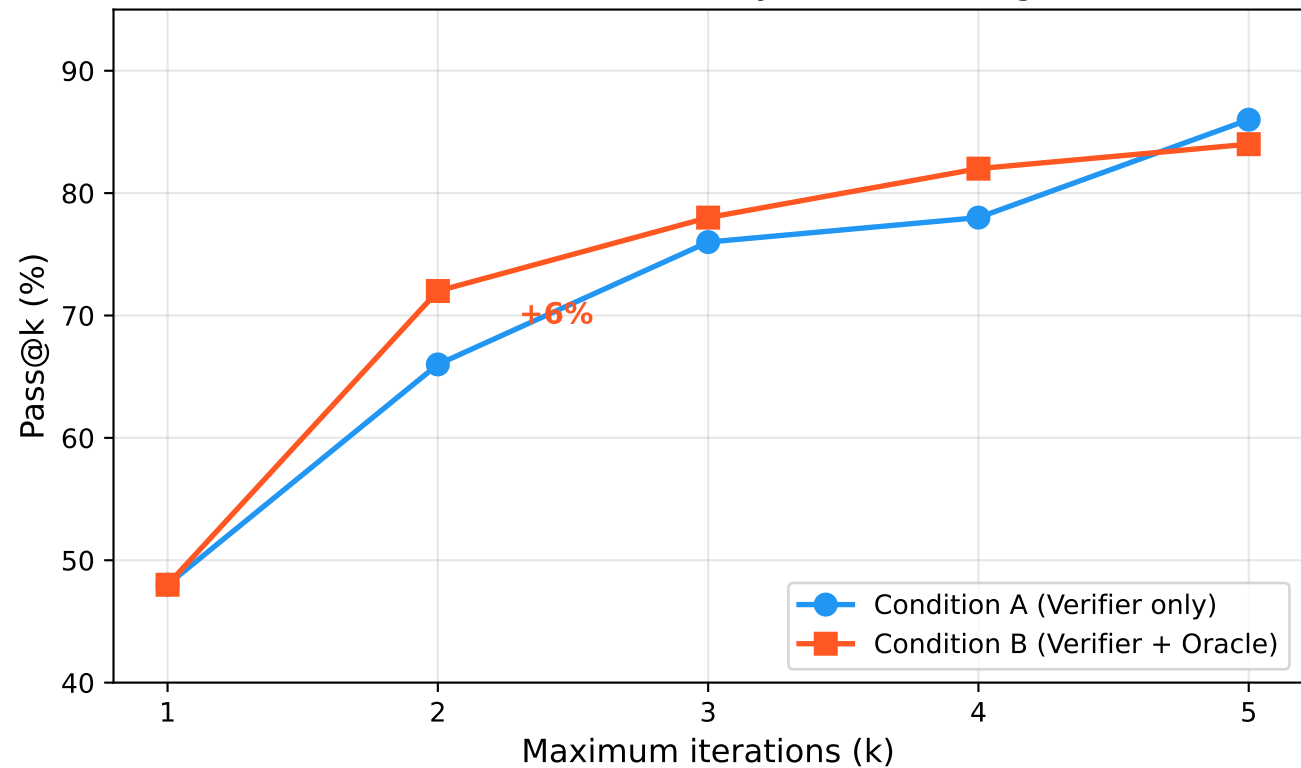
Cumulative Pass Rate by Iteration Budget
