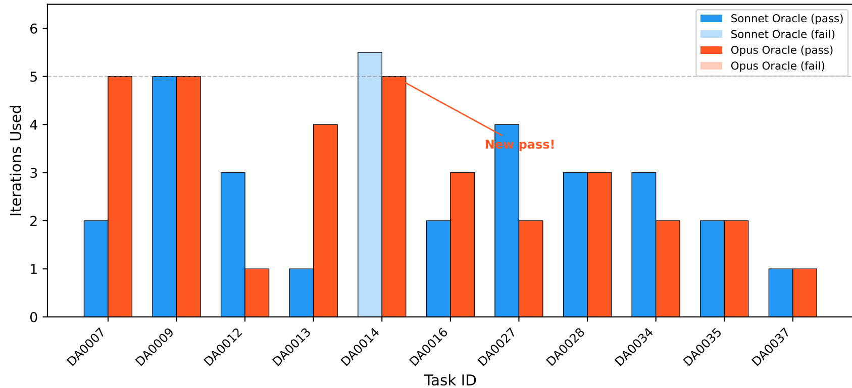
Sonnet Oracle vs Opus Oracle on Hard Tasks (Condition B)
