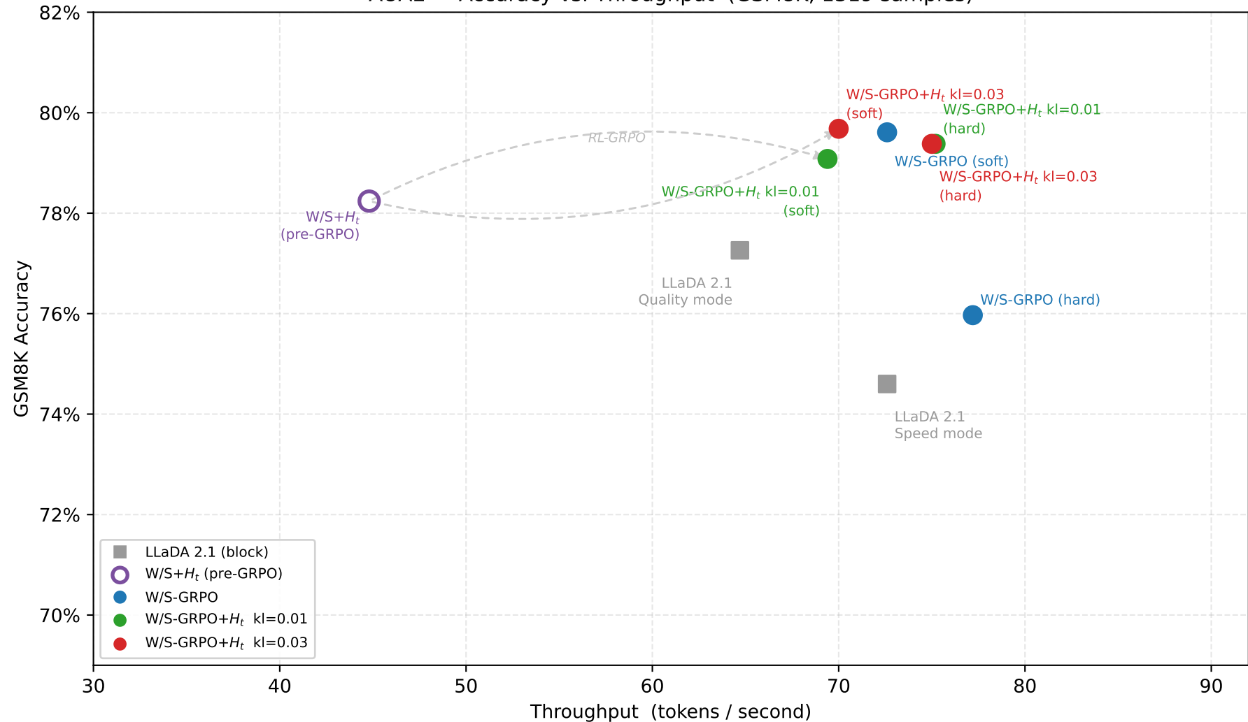
AOAE — Accuracy vs. Throughput (GSM8K, 1319 samples)
