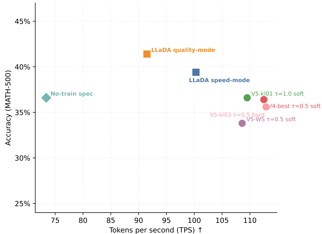
MATH-500: Block-wise Baselines vs. Trained AOA (any-order)
