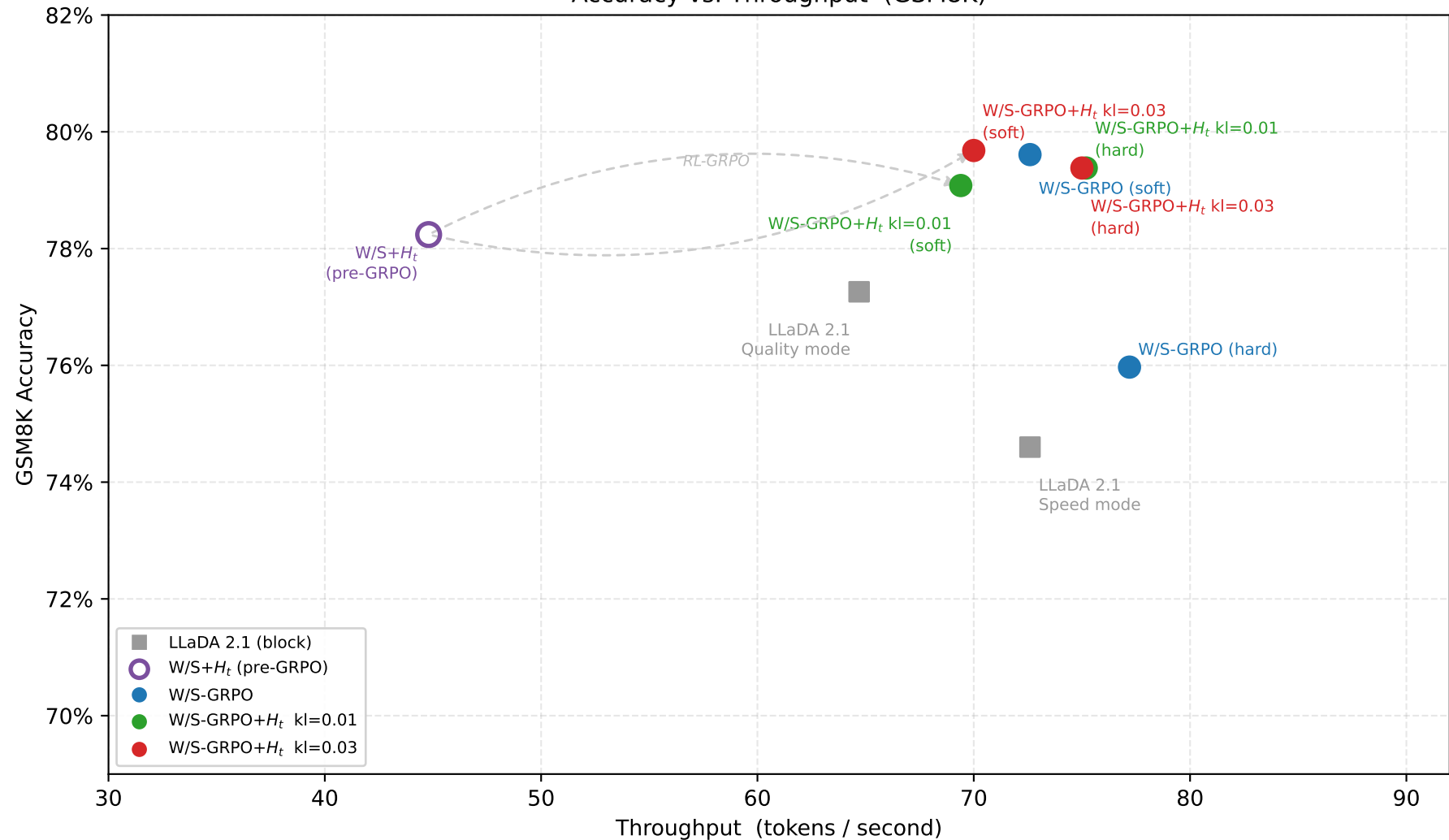
Accuracy vs. Throughput (GSM8K)
