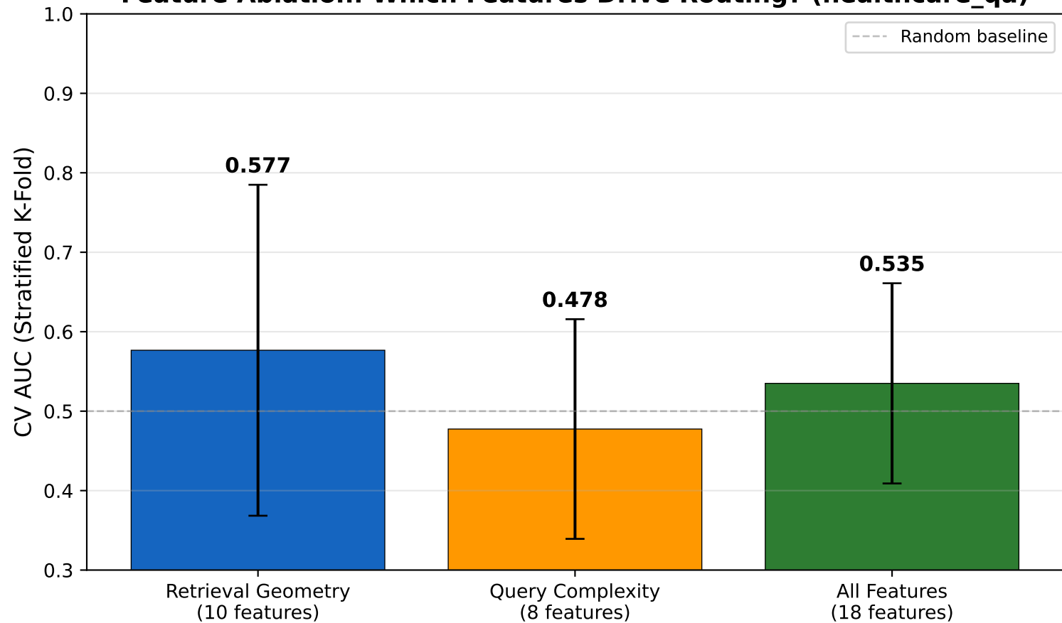
Feature Ablation: Which Features Drive Routing? (healthcare_qa)
