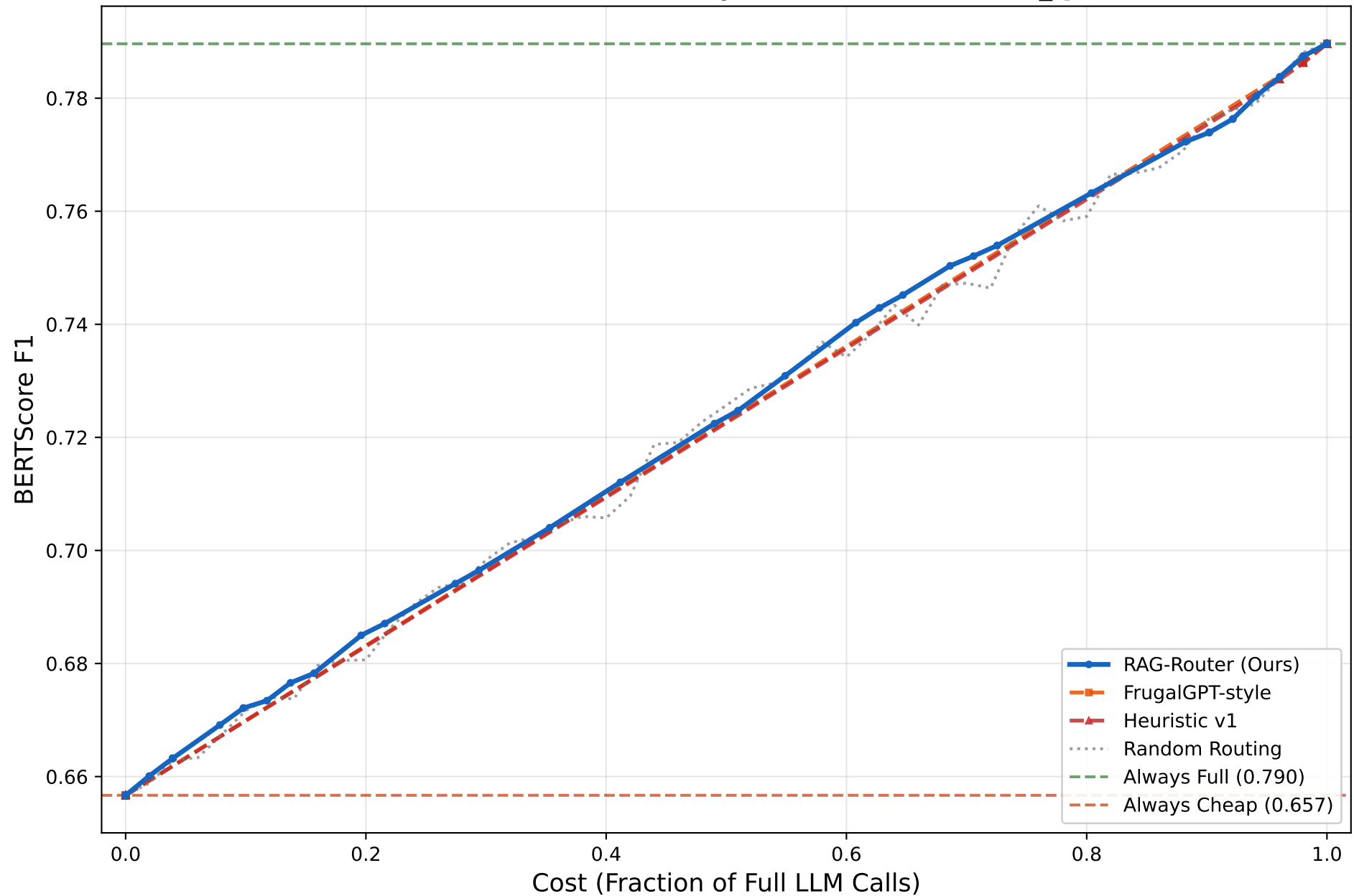
Pareto Frontier: Accuracy vs Cost (healthcare_qa)
