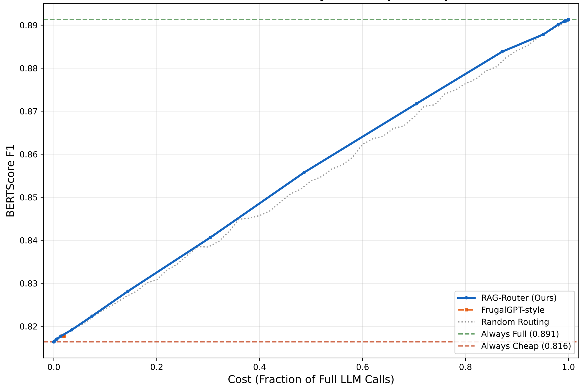
Pareto Frontier: Accuracy vs Cost (pubmedqa)
