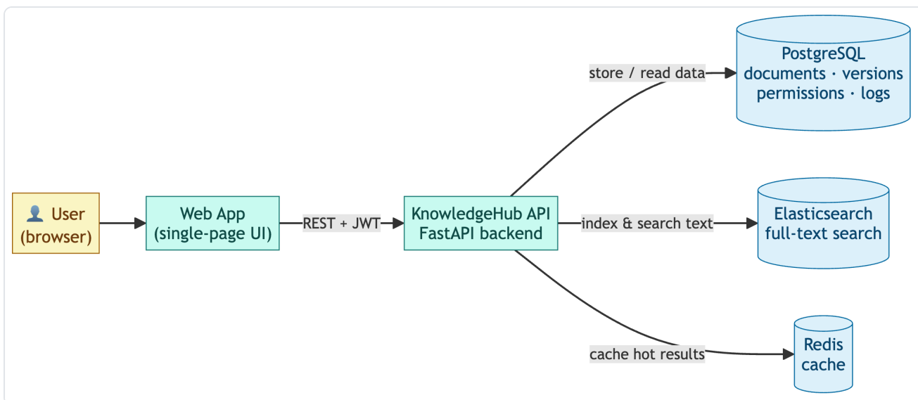
Figure 1 — At its simplest: a user works in the Web App, which calls the KnowledgeHub API over REST (secured with JWT). The API uses three data stores — PostgreSQL as the system of record, Elasticsearch for fast full-text search, and Redis to cache hot results.
