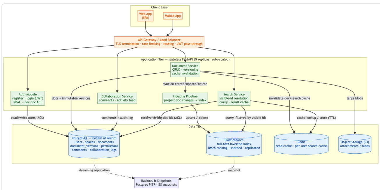
Figure 2 — Components, modules, and their interactions. The application tier is stateless and horizontally scaled; PostgreSQL is the system of record while Elasticsearch and Redis are independently scalable derived stores.
