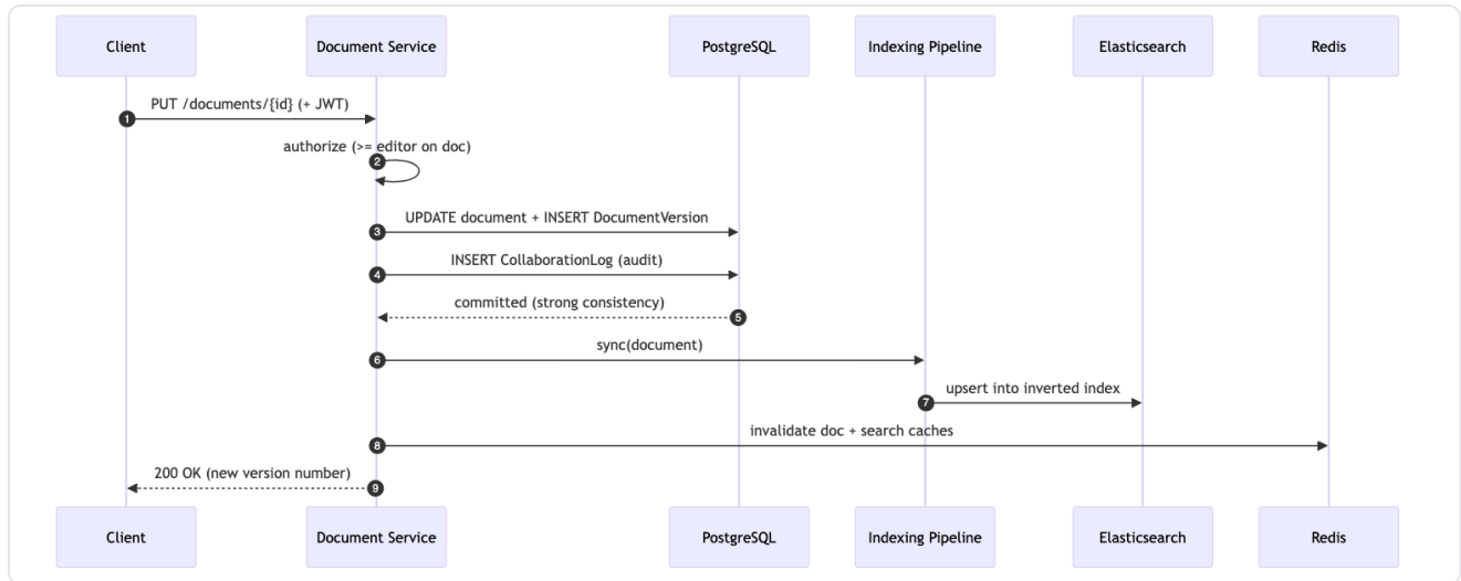
Figure 3 — A document edit is committed to PostgreSQL (row + immutable version + audit log), then projected into the Elasticsearch index, and the affected caches are invalidated.
