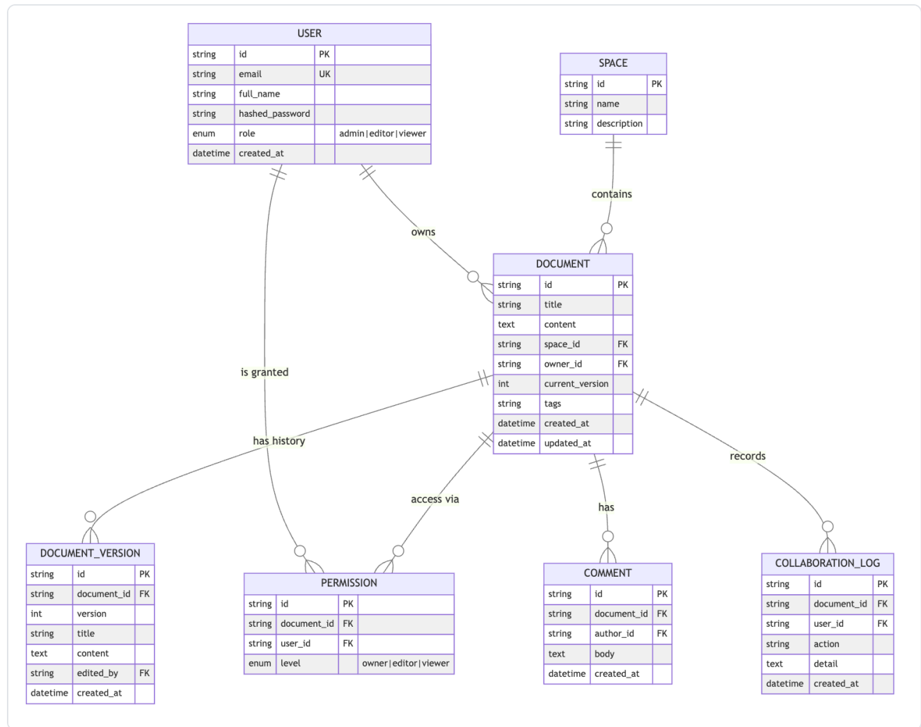
Figure 5 — Relational schema (PostgreSQL). document_versions is append-only for full revision history; permissions is the per-document ACL; collaboration_logs is the append-only audit trail.
