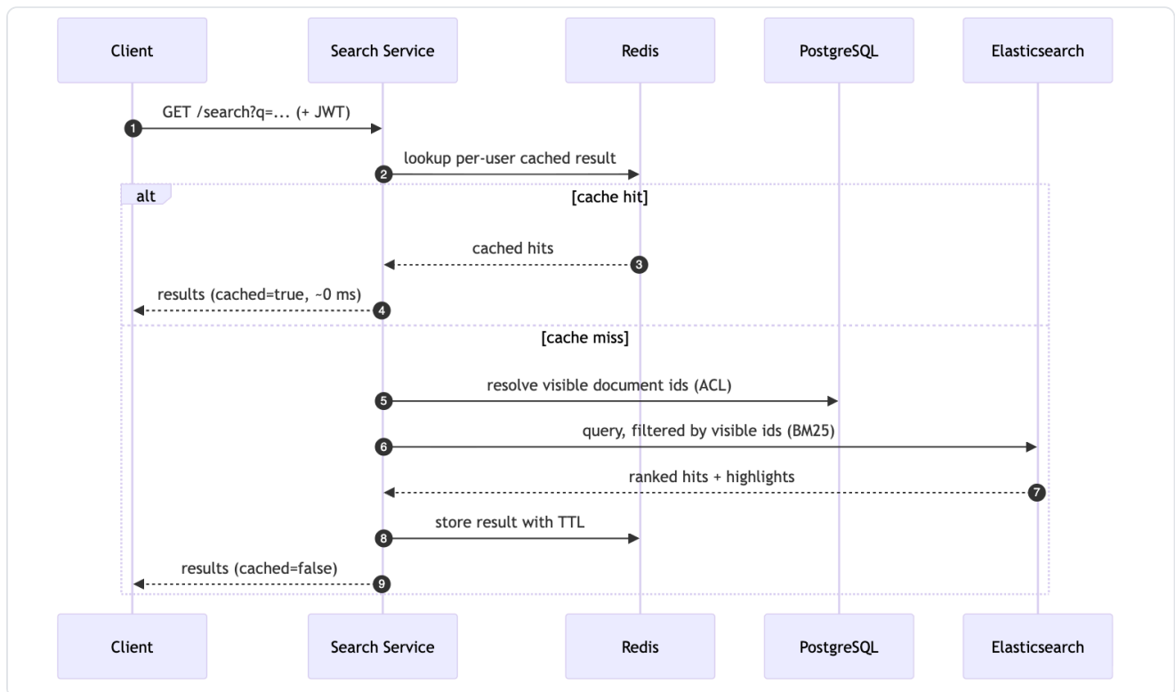
Figure 4 — Search first consults the per-user Redis cache; on a miss it resolves the caller's visible document IDs from the ACL, queries Elasticsearch filtered to those IDs, then caches the result.
