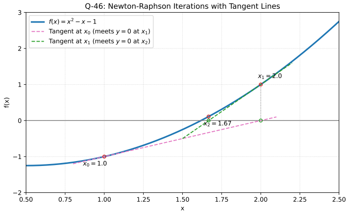
Fig. 1.2.9.1. Newton-Raphson iteration for f(x) = x^2 - x - 1
