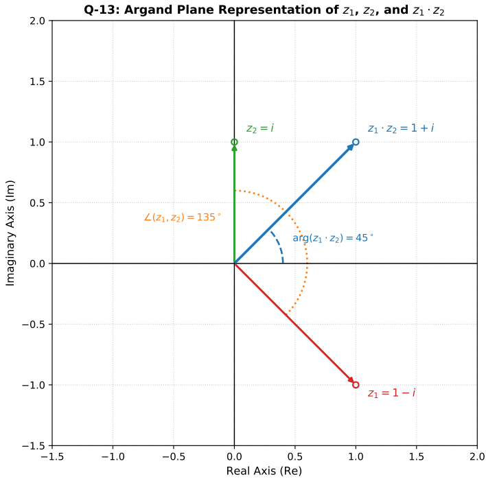
Fig. 1.2.2.1. Complex-plane representation of z_1 z_2
