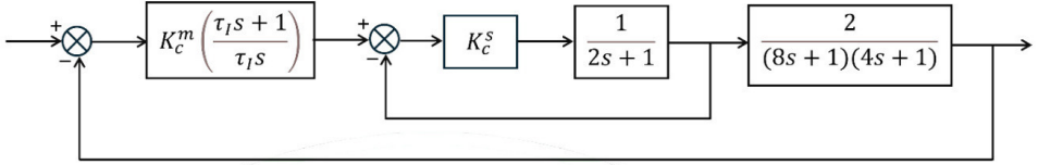
Fig. 1.2.11.1. Series cascade control system given in GATE CH 2025 Q62
