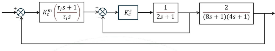
Fig. 1.2.11.1. Series cascade control system given in GATE CH 2025 Q62
