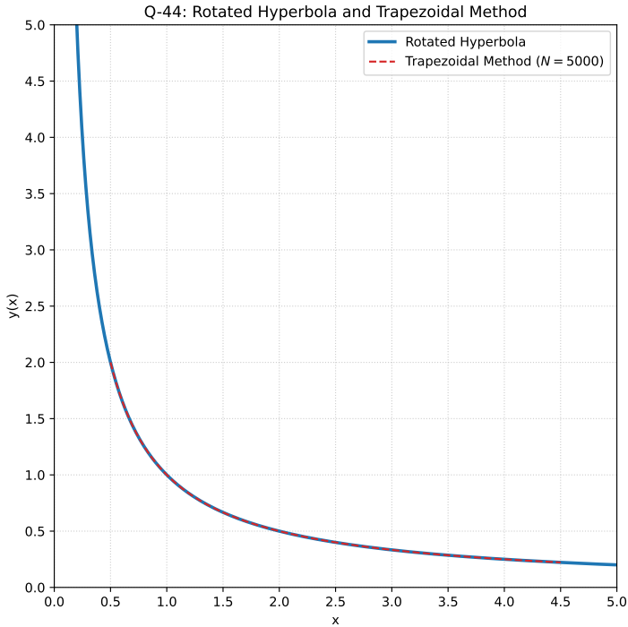
Fig. 1.2.7.1. Numerical solution of the differential equation.
