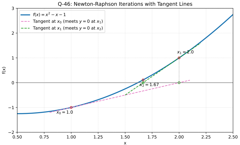
Fig. .5. Newton-Raphson iteration for f(x) = x^2 - x - 1
