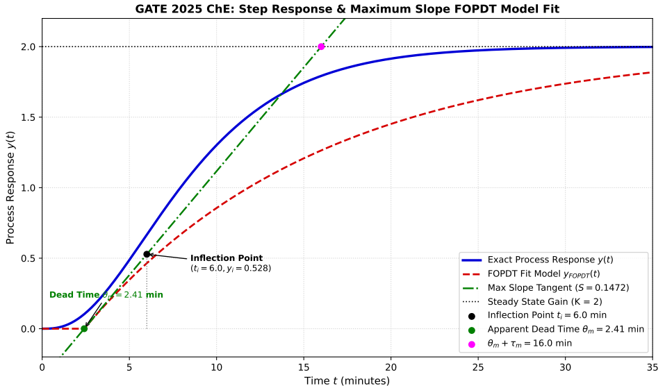
Fig. .6. Maximum-slope FOPDT approximation of the given process response
