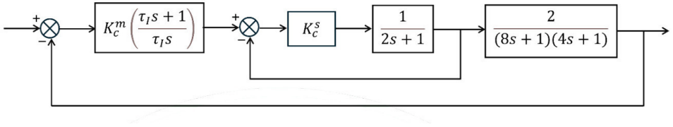
Fig. .7. Series cascade control system given in GATE CH 2025 Q62
