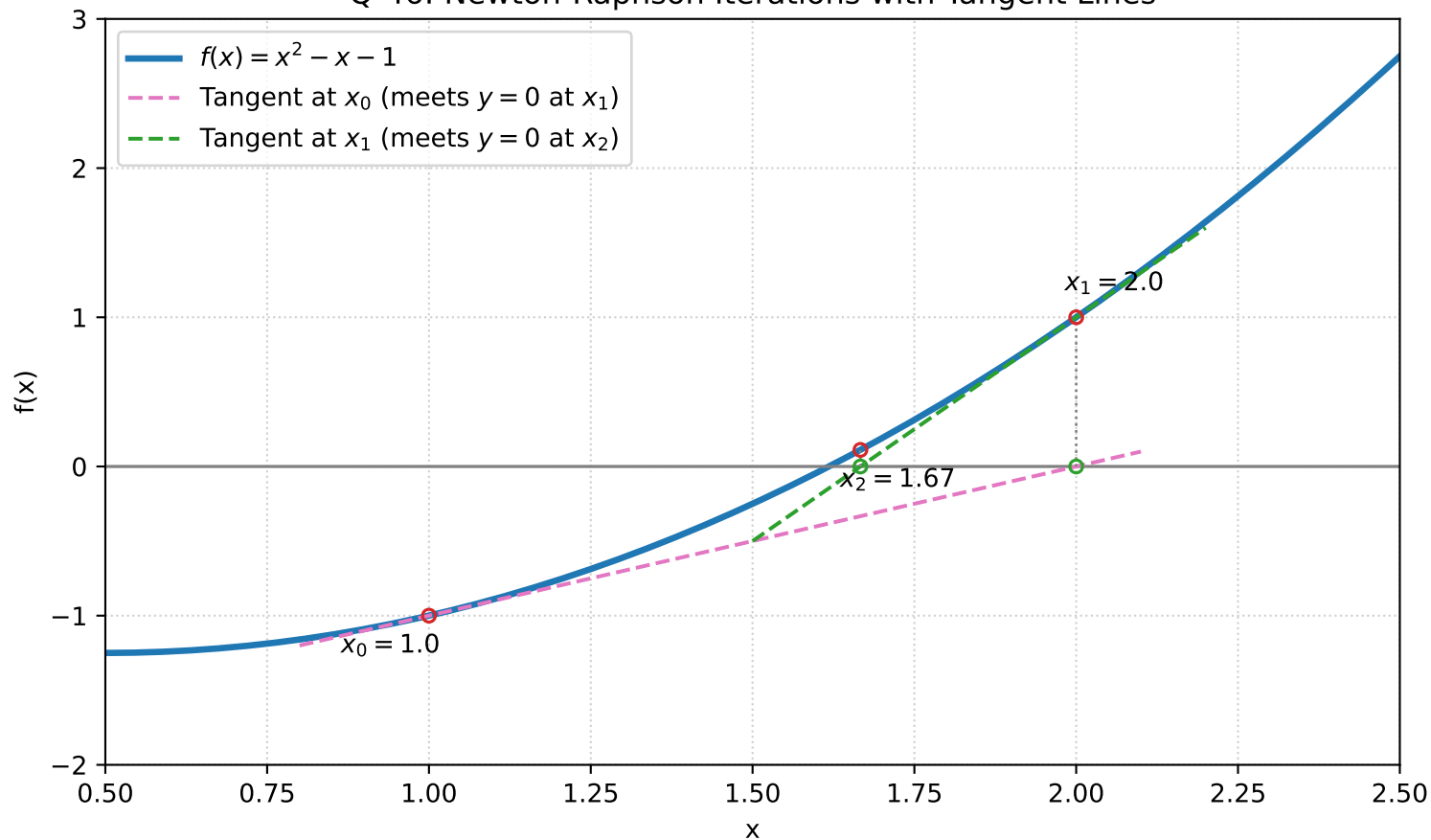
Q-46: Newton-Raphson Iterations with Tangent Lines
