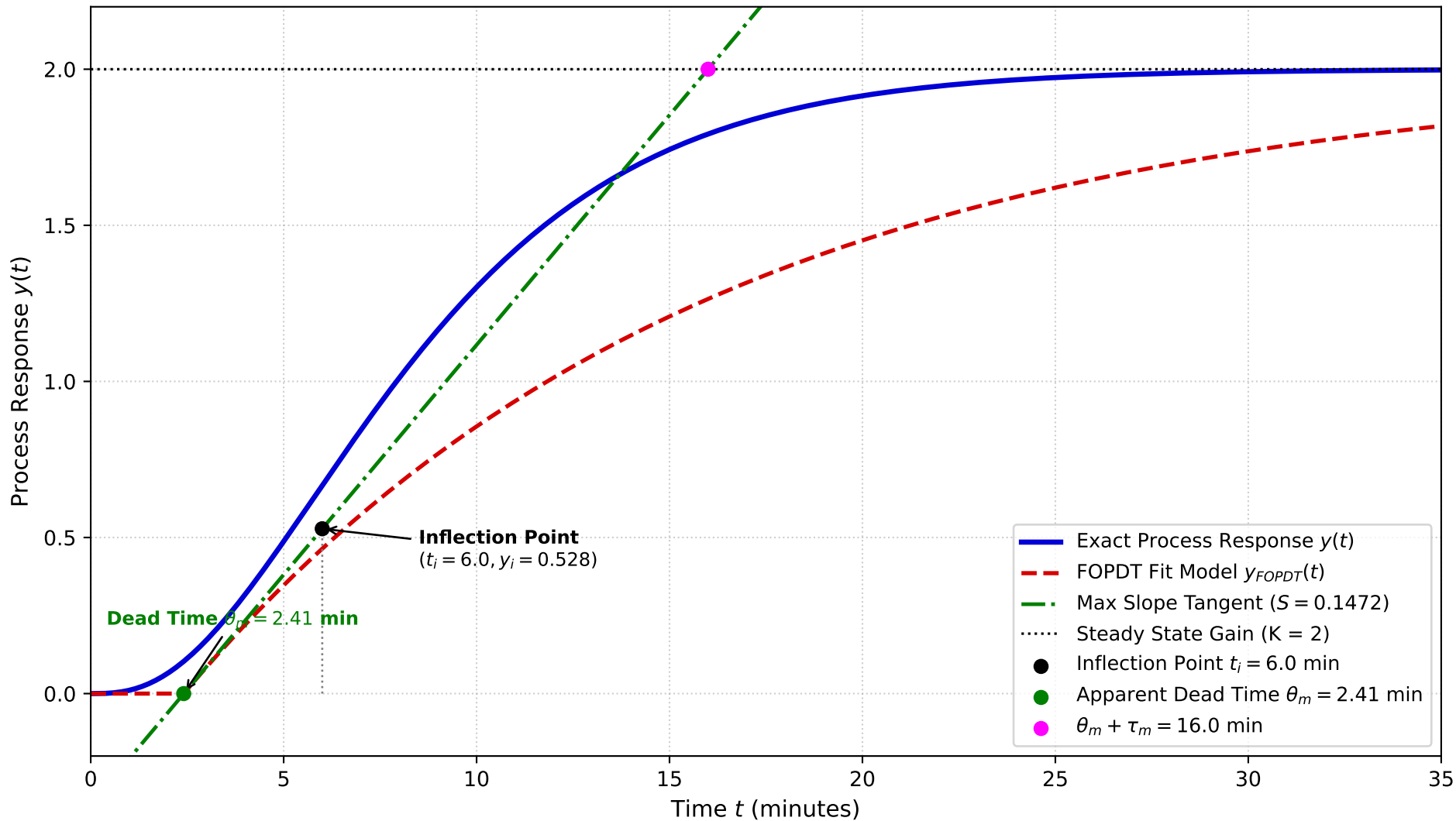
GATE 2025 ChE: Step Response & Maximum Slope FOPDT Model Fit
