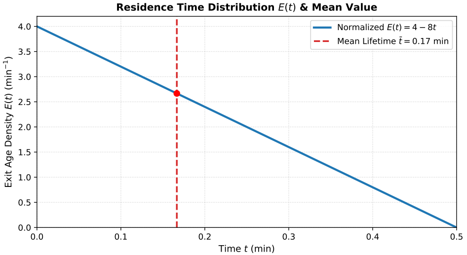
Fig. 1.2.4.1. Residence time distribution E(t) for the given reactor
