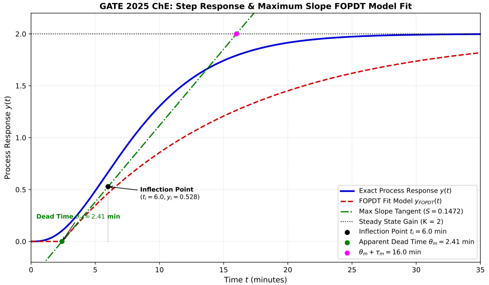
Fig. 1.2.10.1. Maximum-slope FOPDT approximation of the given process response
