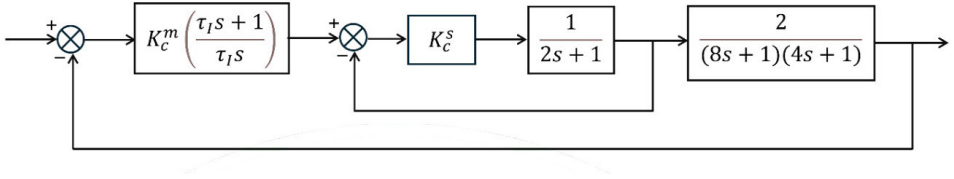
Fig. 1.2.11.1. Series cascade control system given in GATE CH 2025 Q62
