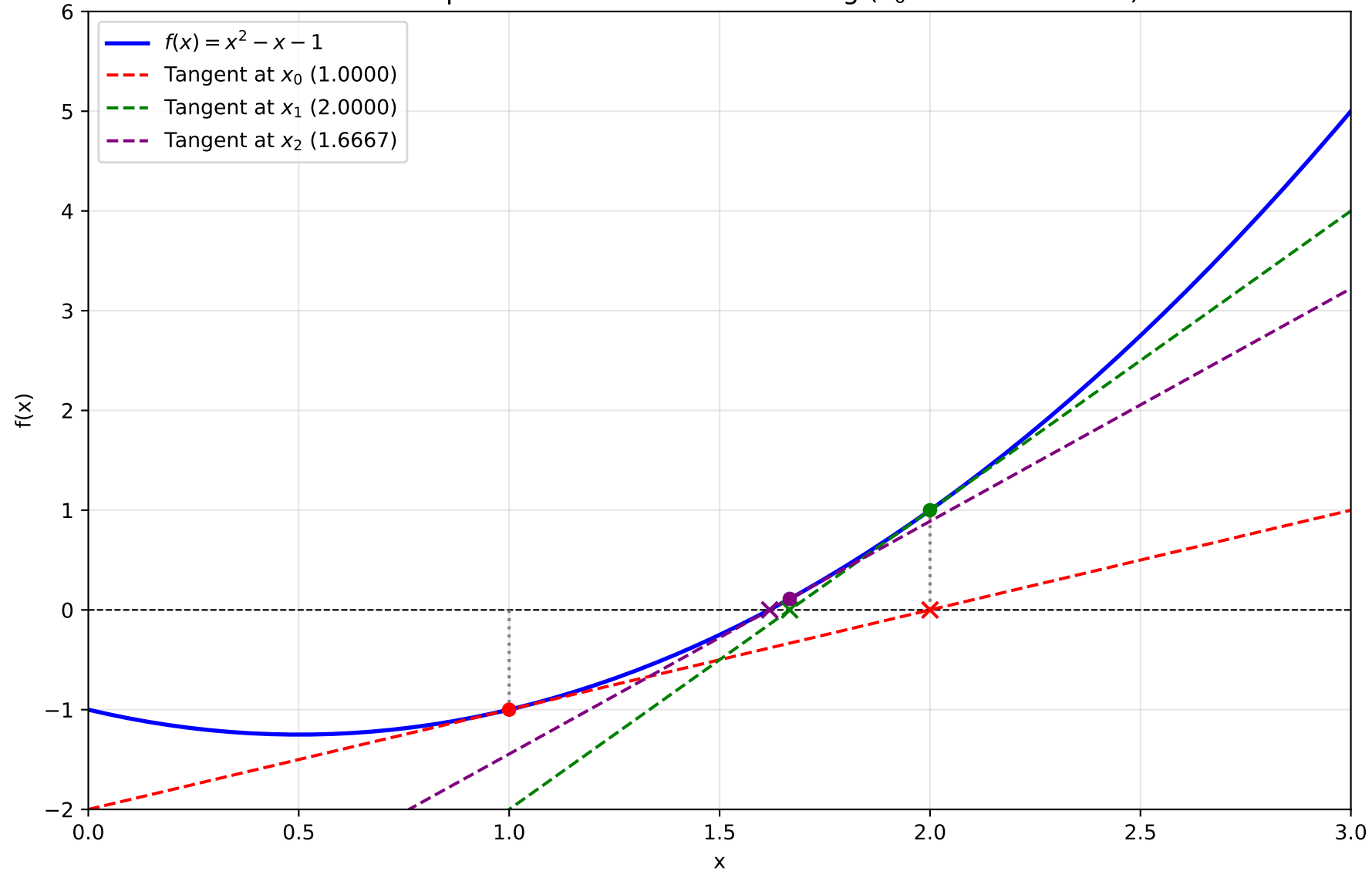
Newton-Raphson Iteration Visual Tracking ( x_0 = 1 to 3 Domain)
