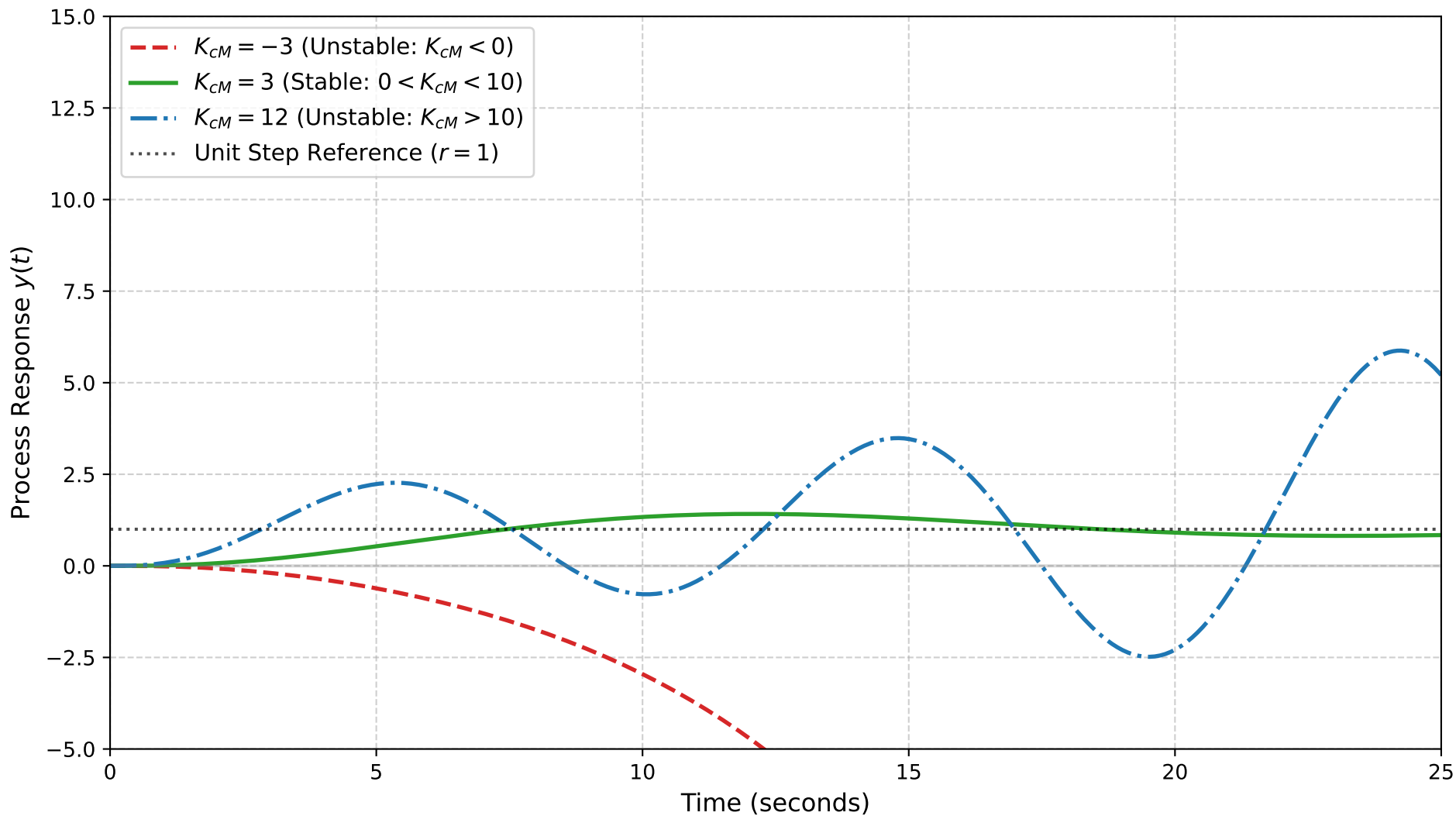
Cascade System Step Response Across Stability Regimes
