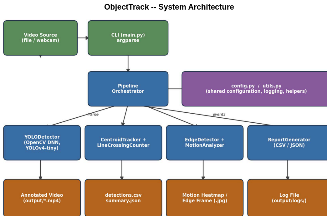
Figure 1: ObjectTrack system architecture.
