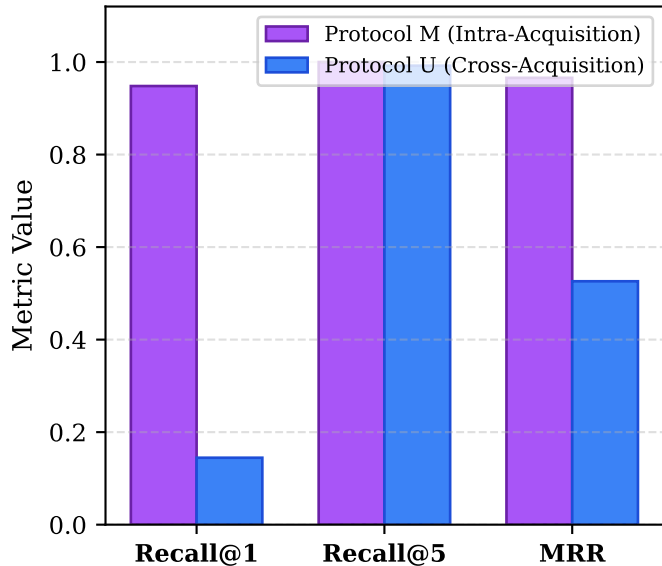
(b) Protocol M vs Protocol U Separation
