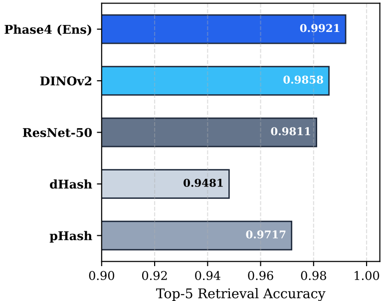
(a) Protocol U Top-5 Accuracy
