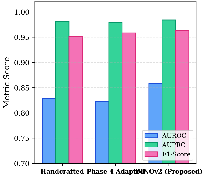
(a) Quality-Risk Screening Performance
