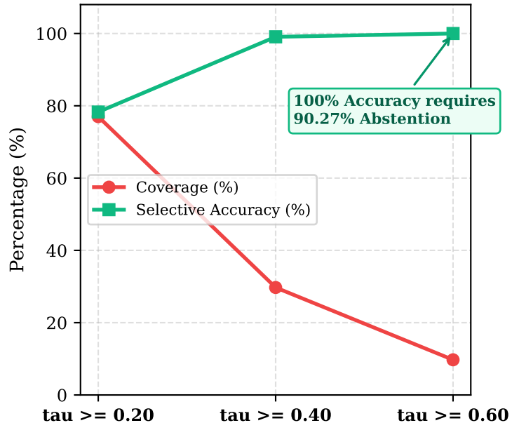
(b) Uncertainty-Aware Selective Prediction
