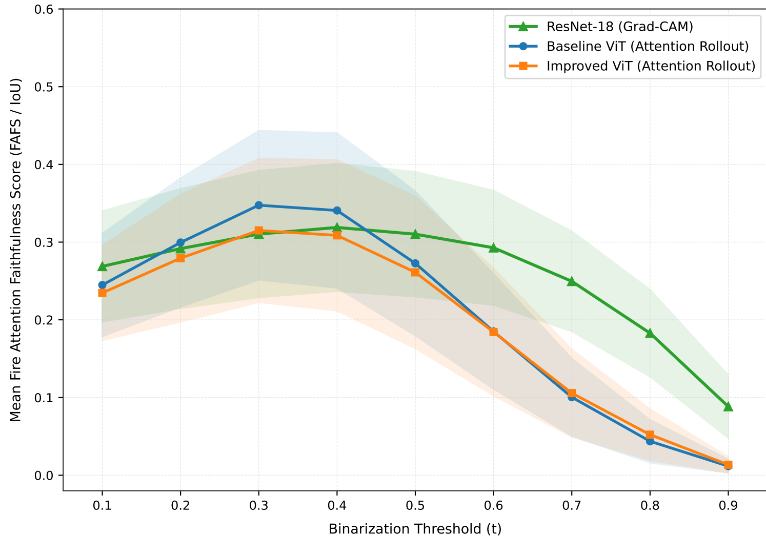
Explainability Spatial Faithfulness (FAFS) Comparison (N=50)
