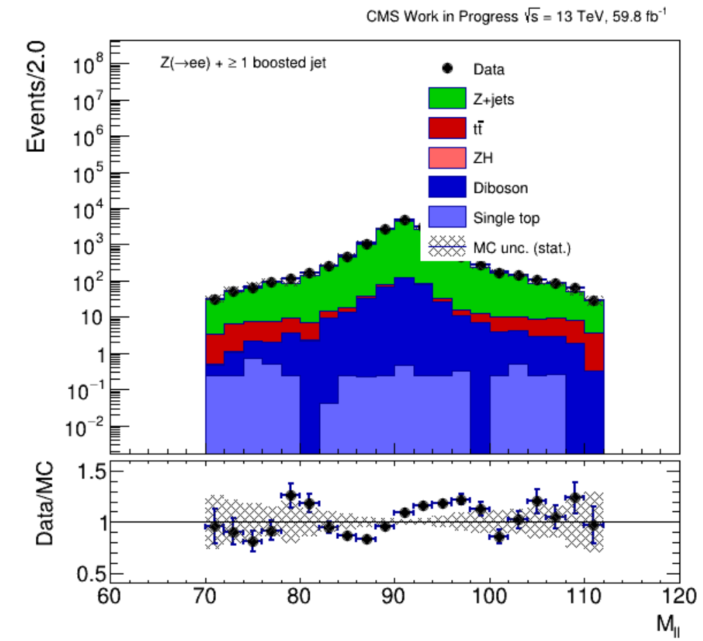
ZMass_Z_jet_Zee_18_amcno.png
