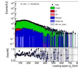
pt_sub0_Z_jet_Zee_18_amcno.png
