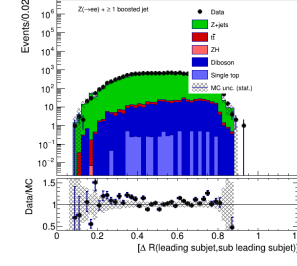
deltaR_subjets_Z_jet_Zee_18_amcno.png
