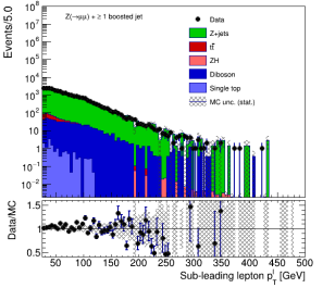
pt_sub1_Z_jet_Zmm_18_amcno.png
