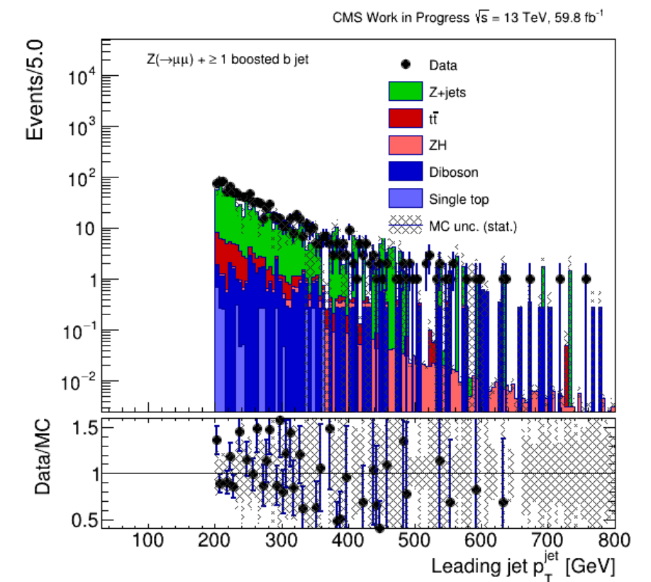
pt_jet_Z_bjet_Zmm_18_amcnlo.png
