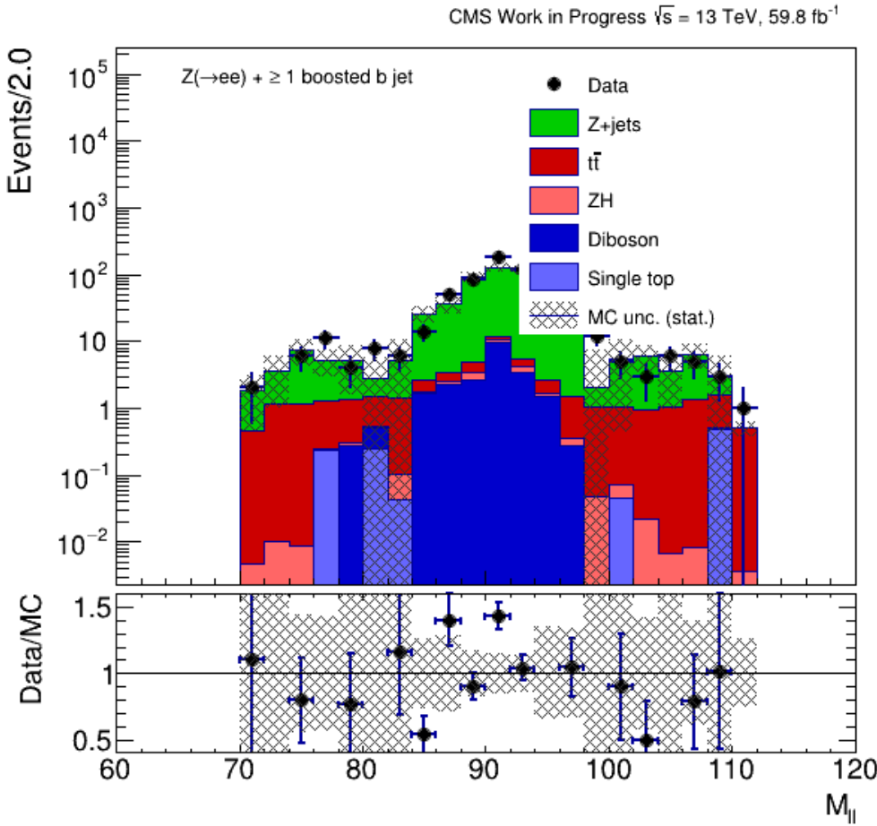
ZMass_Z_bjet_Zee_18_amcno.png
