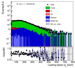
pt_sub0_Z_jet_Zmm_18_amcno.png
