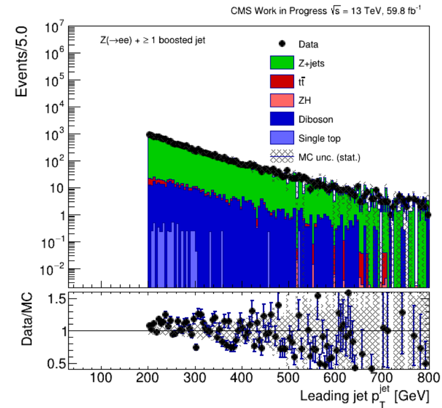
pt_jet_Z_jet_Zee_18_amcnlo.png
