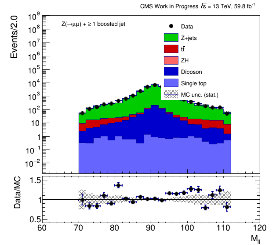
ZMass_Z_jet_Zmm_18_amcno.png
