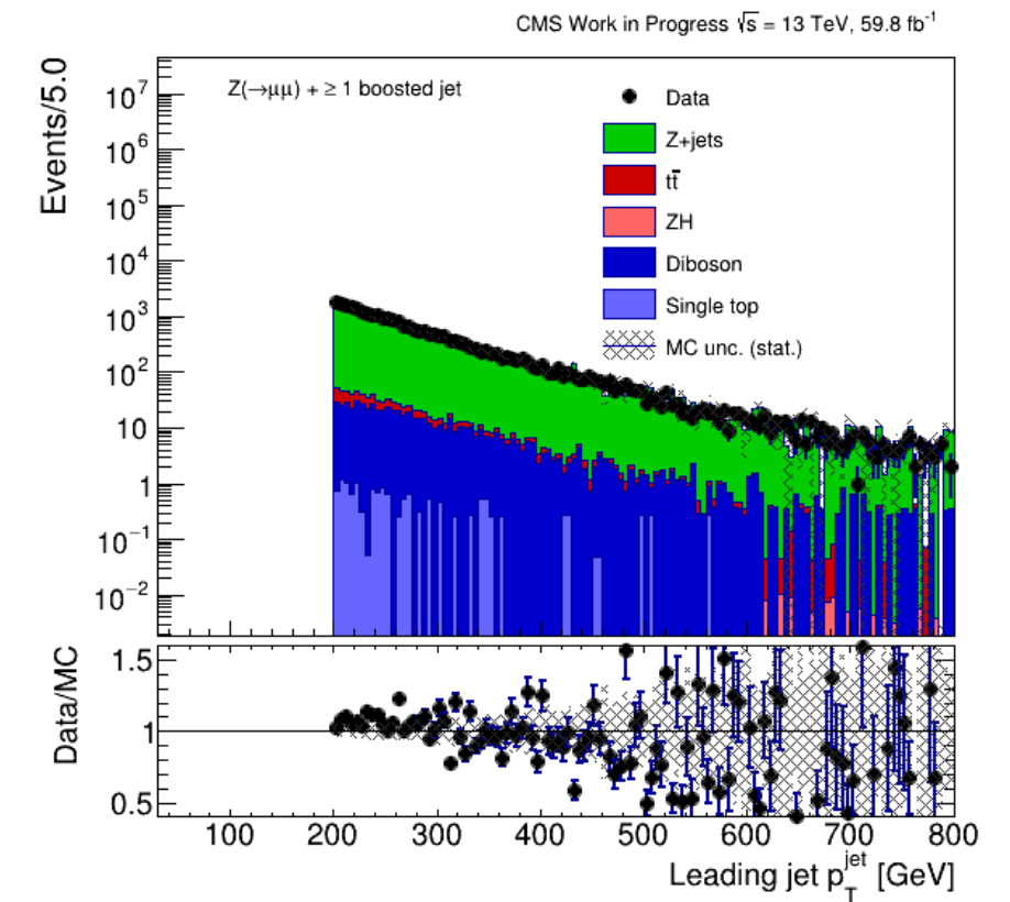
pt_jet_Z_jet_Zmm_18_amcnlo.png
