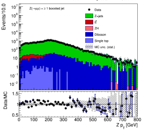
pt_lep1_Z_jet_Zmm_18_amcno.png
