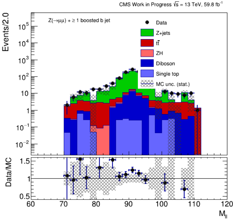
ZMass_Z_bjet_Zmm_18_amcno.png
