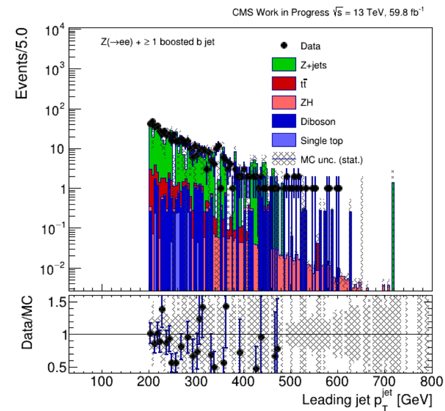
pt_jet_Z_bjet_Zee_18_amcnlo.png
