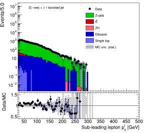
pt_sub1_Z_jet_Zee_18_amcno.png
