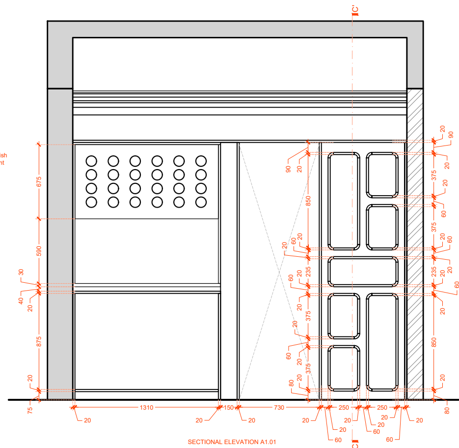
SECTIONAL ELEVATION A1.01
