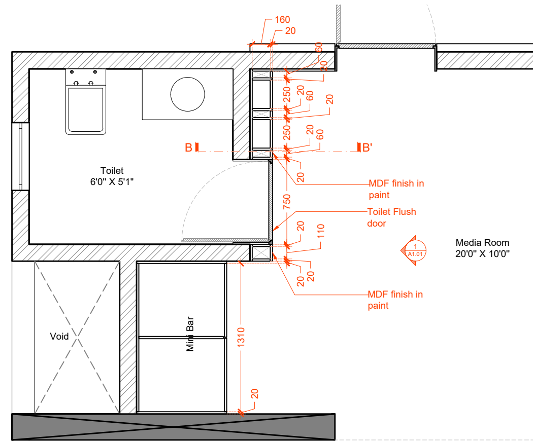
PLAN AT BB'
