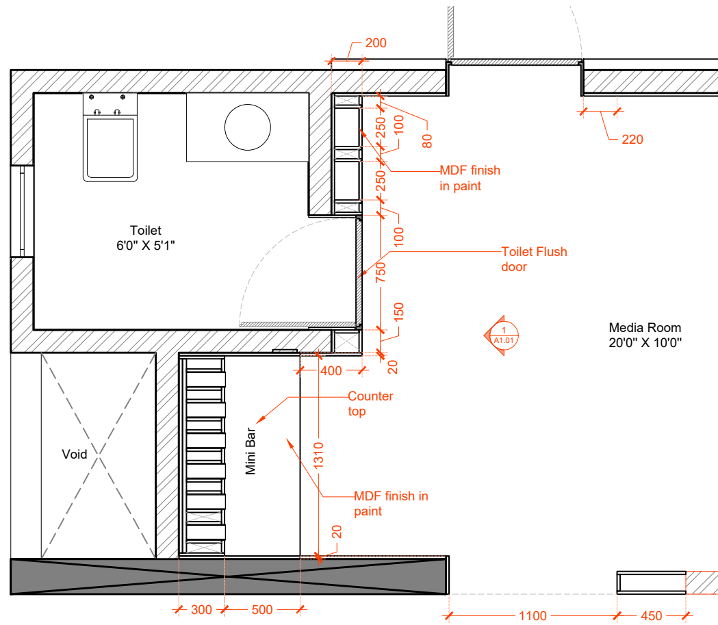
PLAN AT AA'
