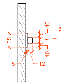
SECTION OF A2.01
