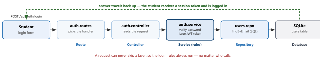
Figure 4.2 — How one login request flows through the layers.
