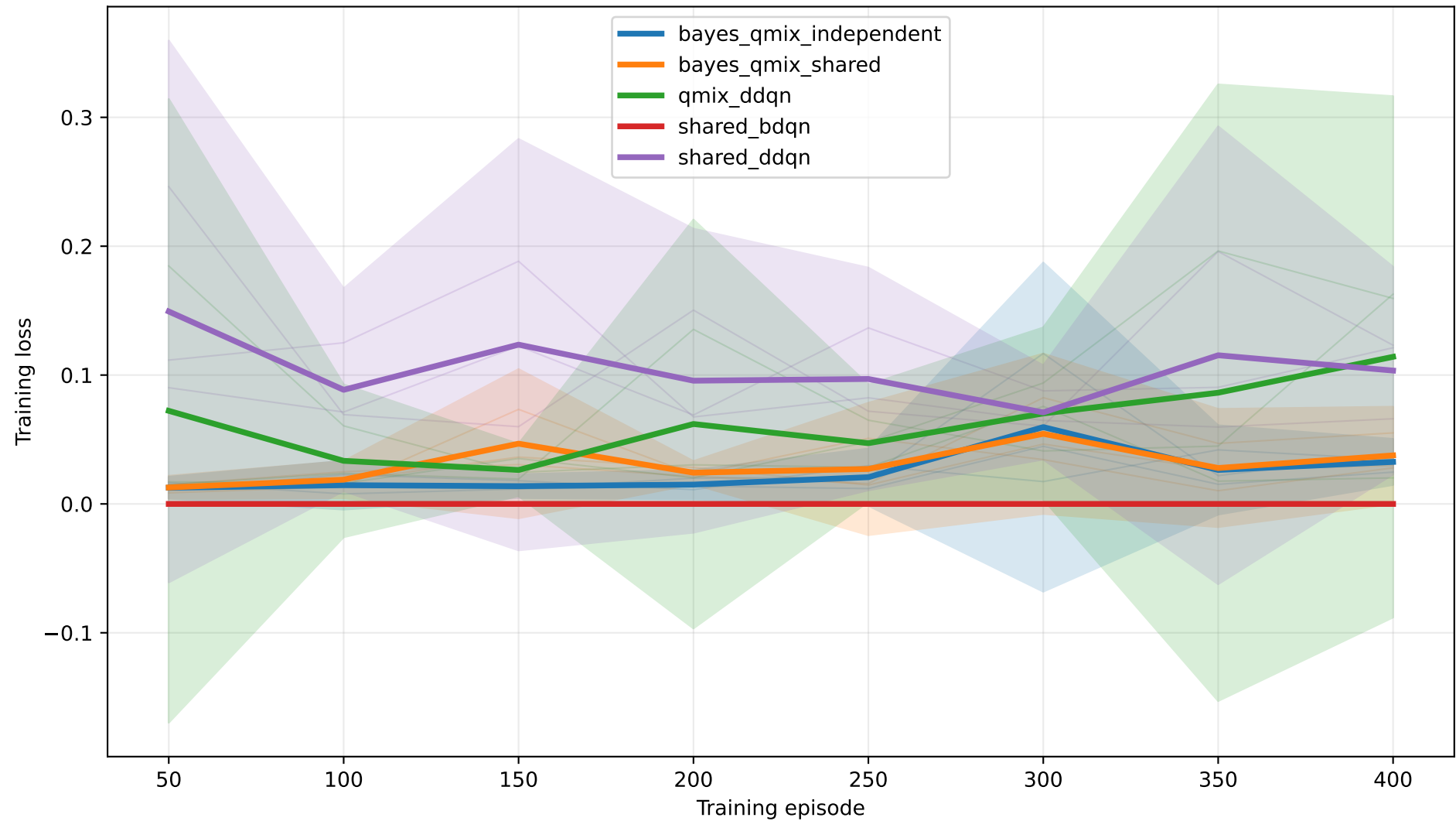
multi — pD=0.70 — Training loss
