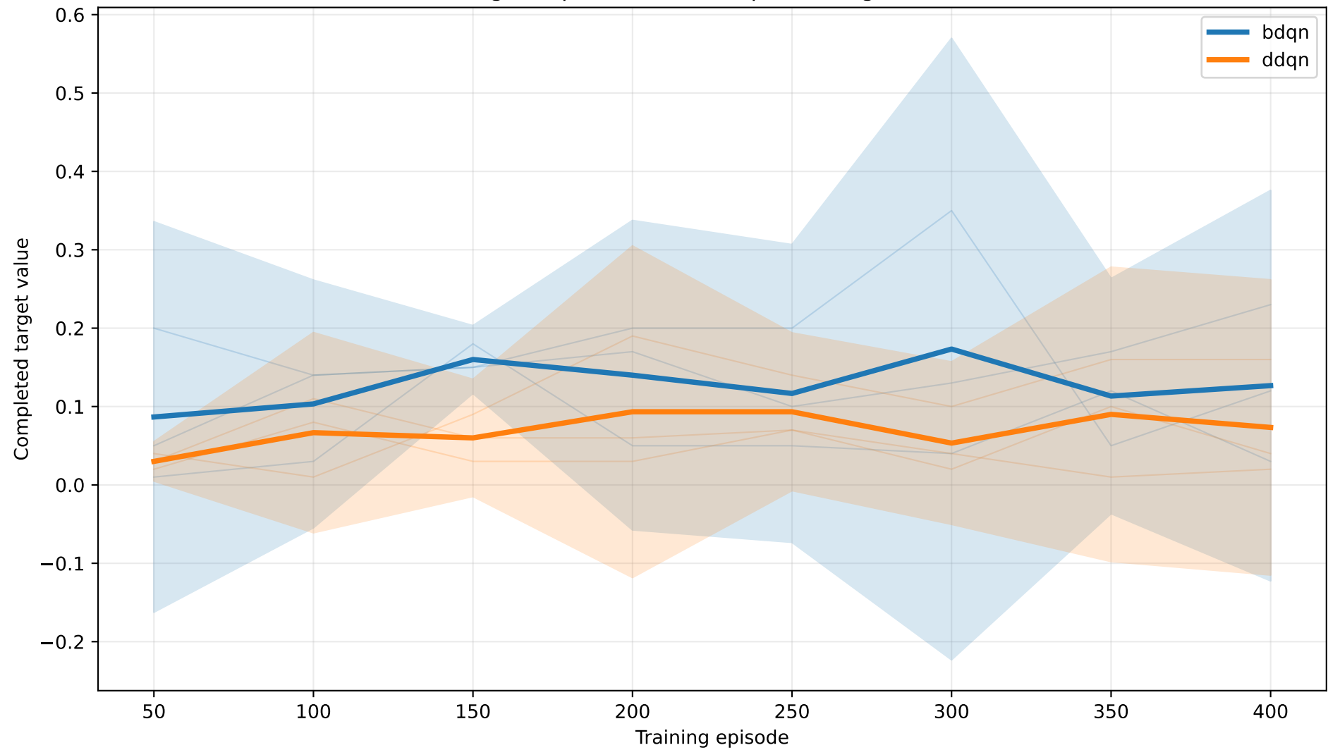
single — pD=1.00 — Completed target value
