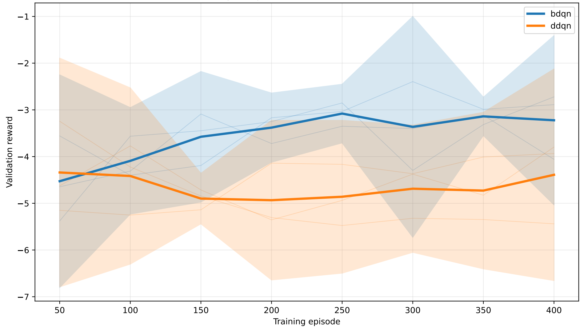
single — pD=1.00 — Validation reward
