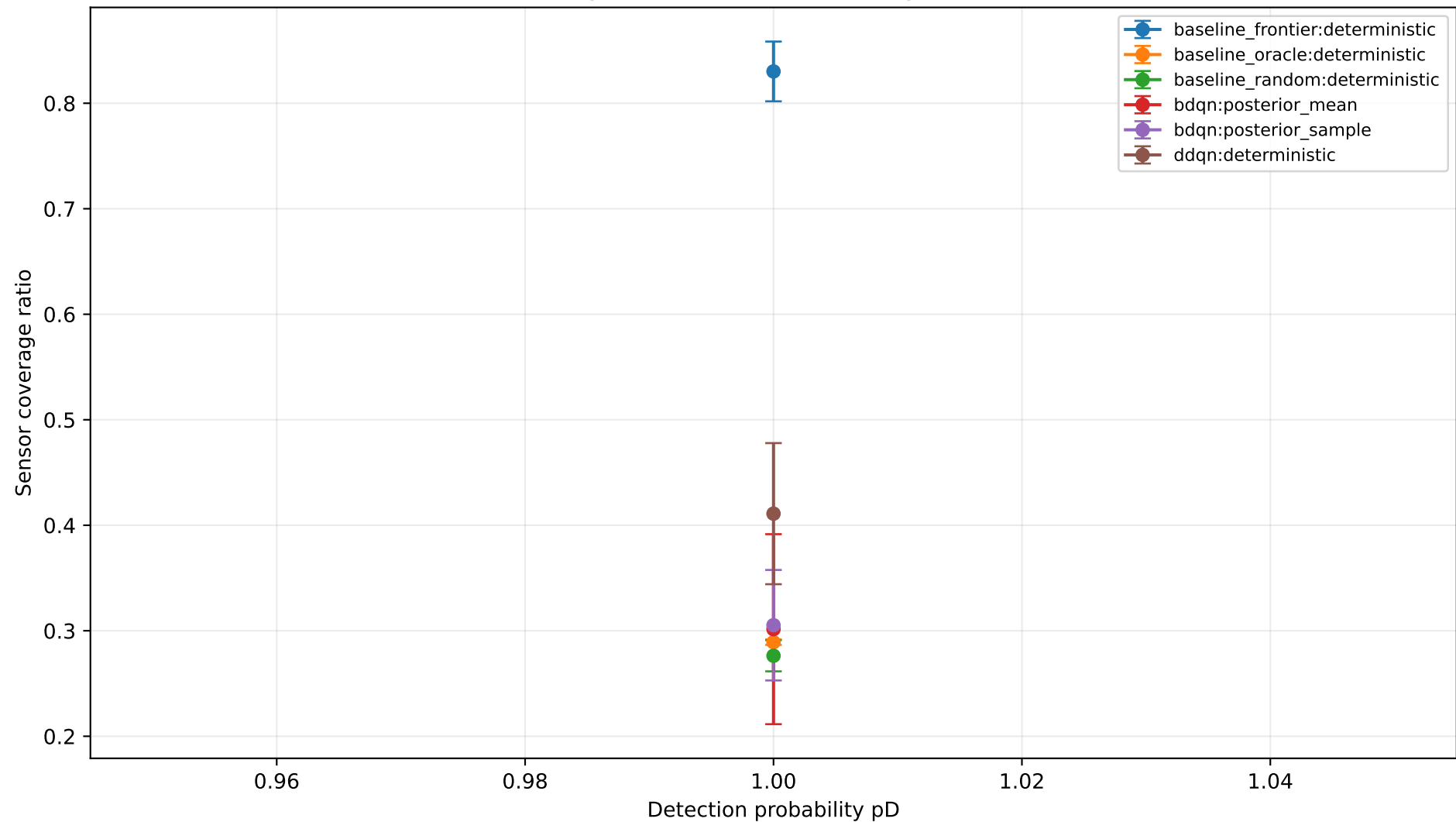
single — final Sensor coverage ratio
