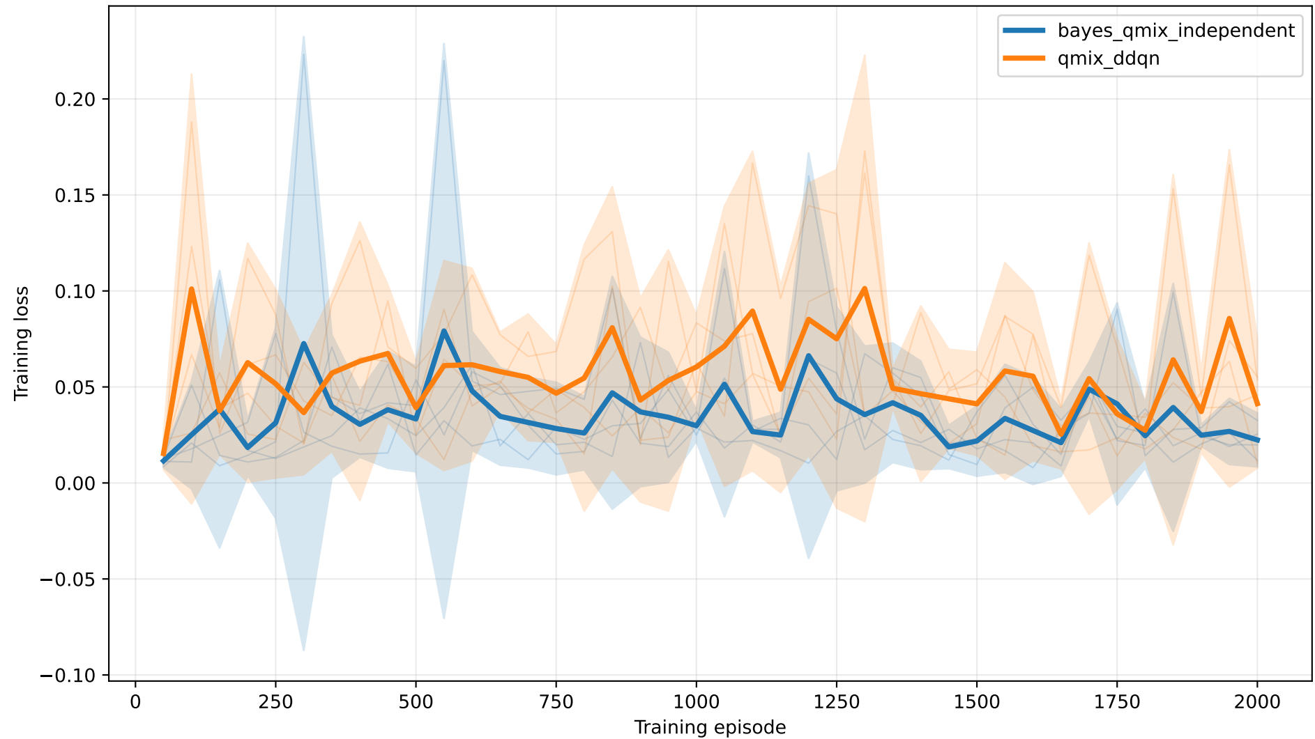
multi — pD=0.50 — Training loss
