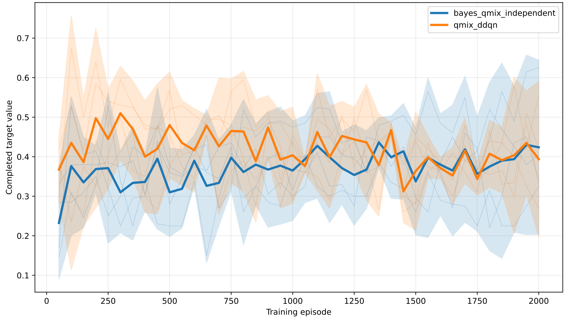
multi — pD=0.50 — Completed target value
