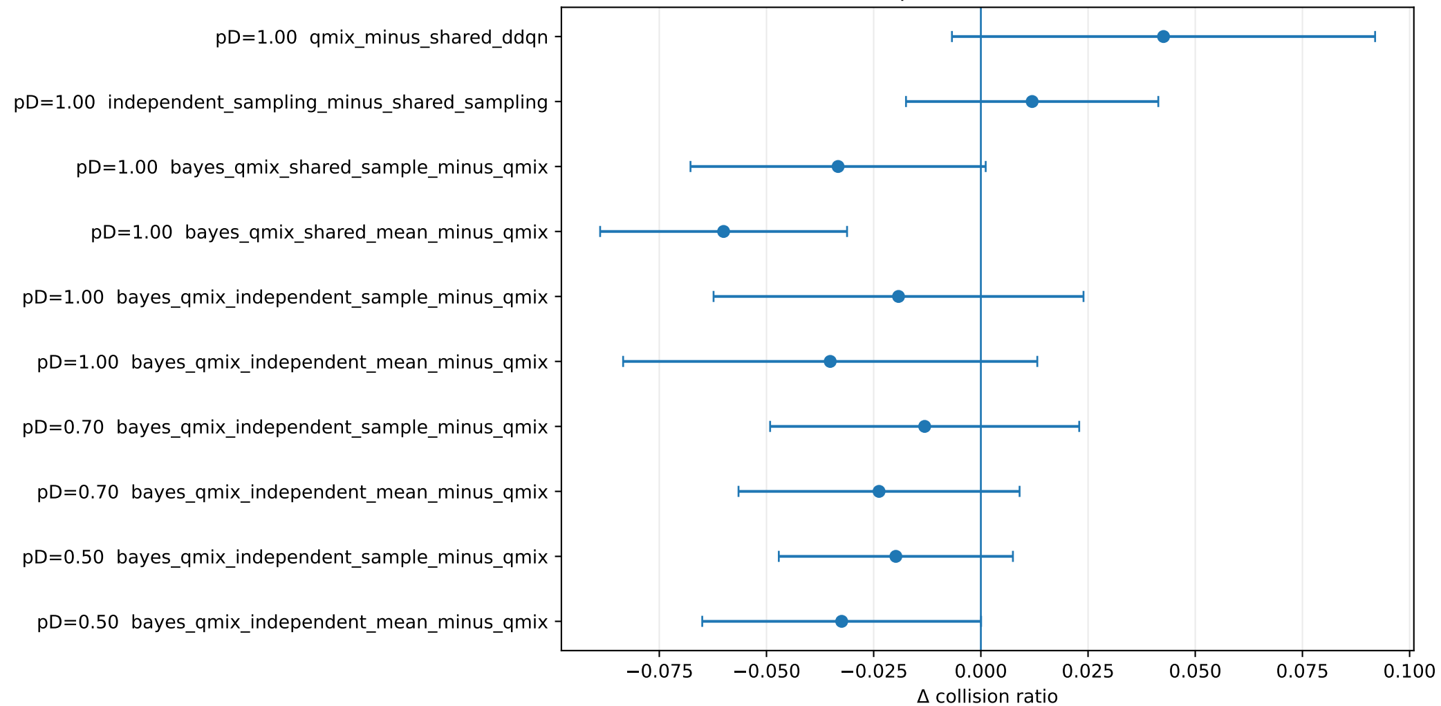
Paired comparisons — \Delta collision ratio
