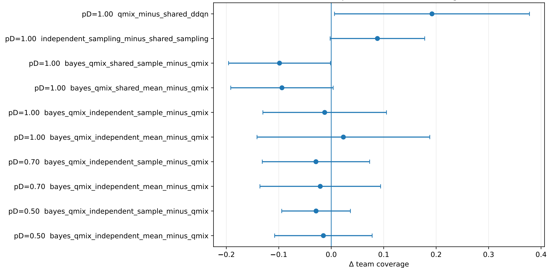
Paired comparisons — \Delta team coverage
