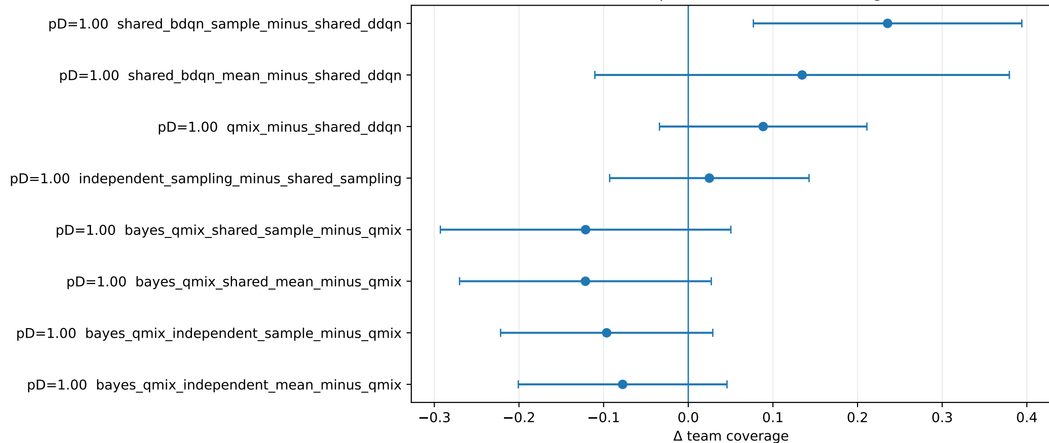
Paired comparisons — \Delta team coverage
